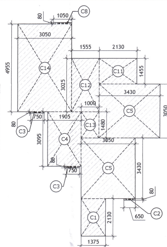
CARPET AREA DIAGRAM 2 BHK (TYPE III)
