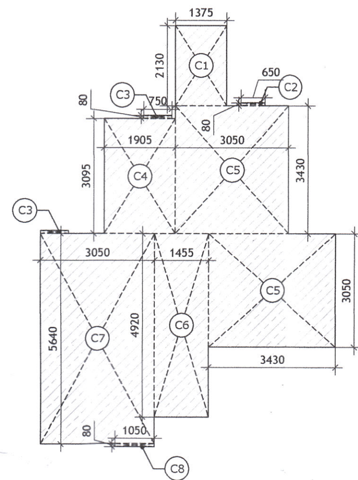
CARPET AREA DIAGRAM 2 BHK (TYPE I)
