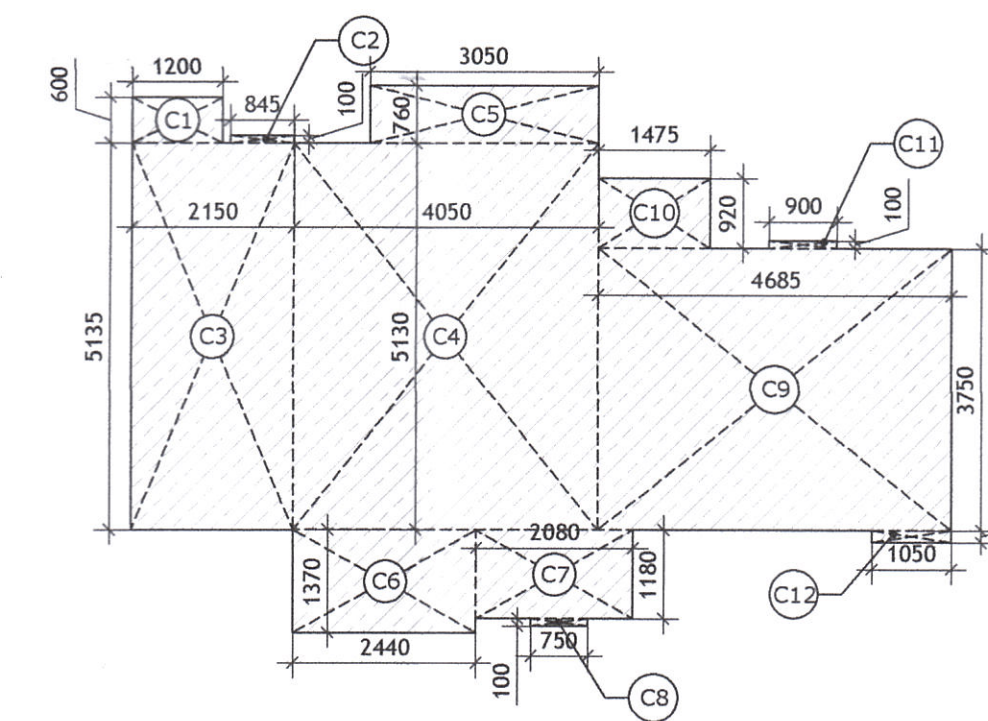
CARPET AREA DIAGRAM 2BHK + STORE (TYPE V)
