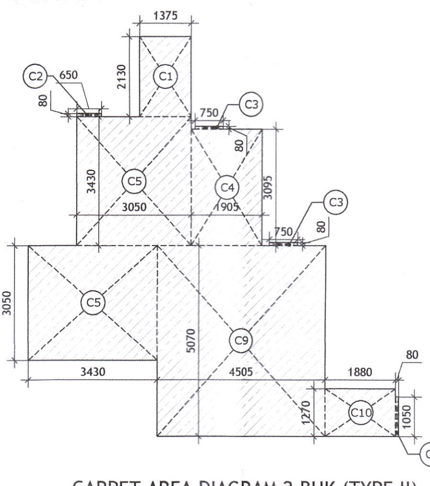
CARPET AREA DIAGRAM 2 BHK (TYPE II)
