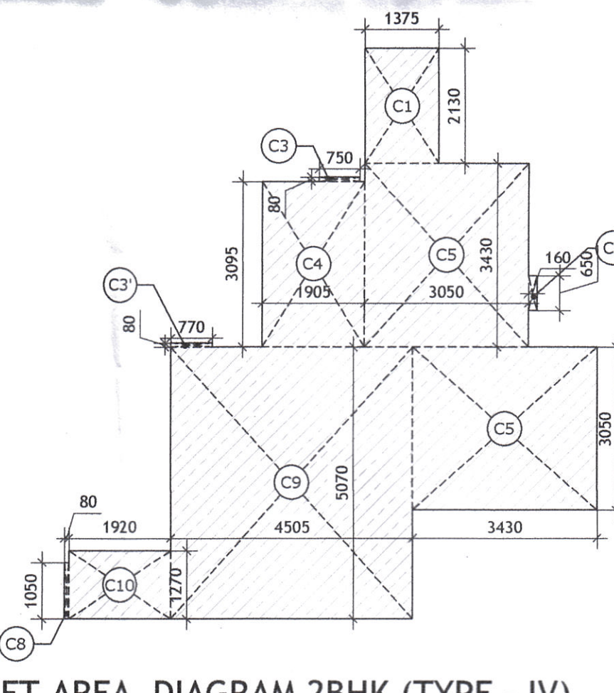
CARPET AREA DIAGRAM 2BHK (TYPE - IV)
