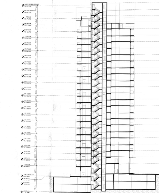
SECTION A
