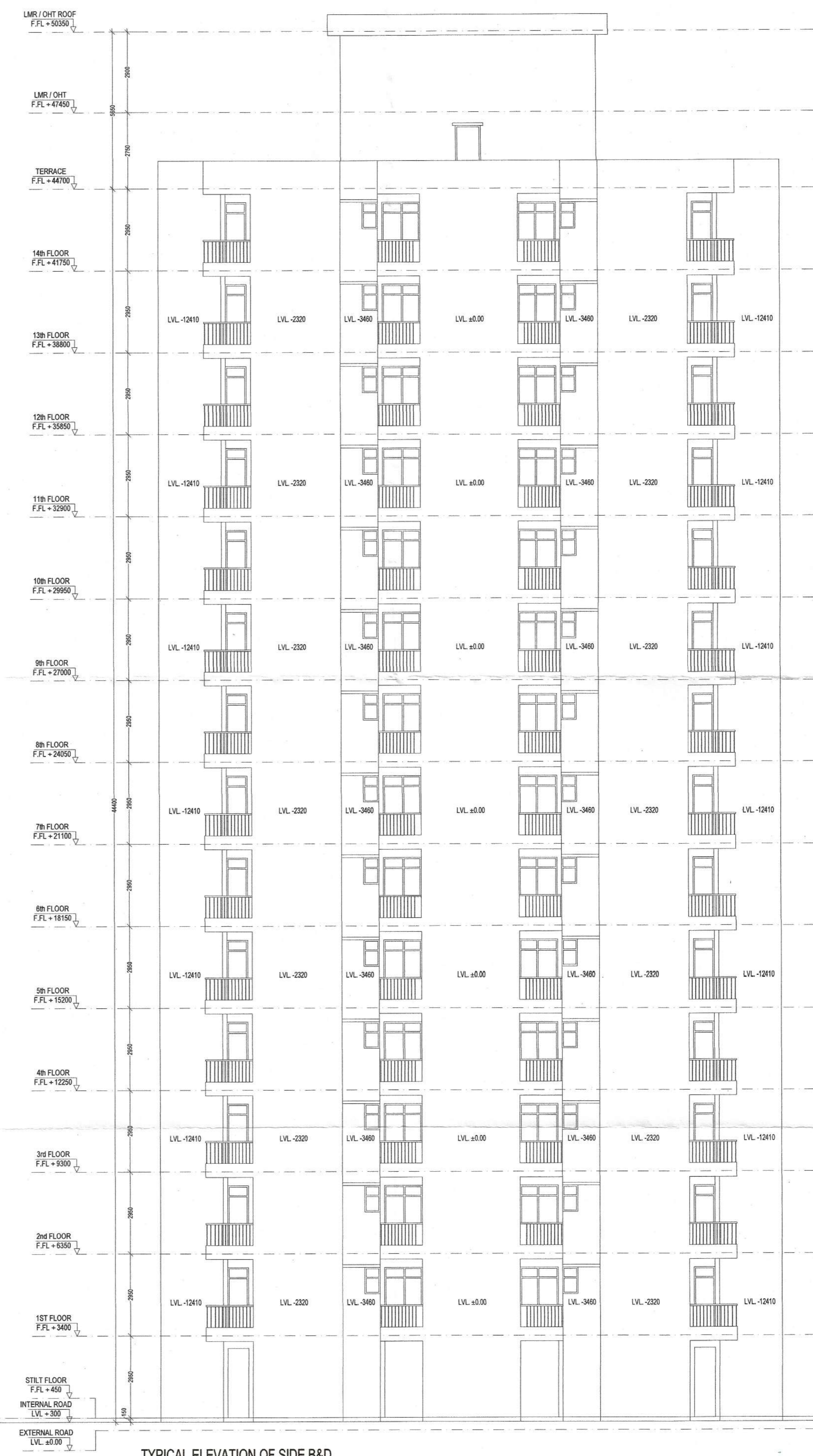
TYPICAL ELEVATION OF SIDE B&D
