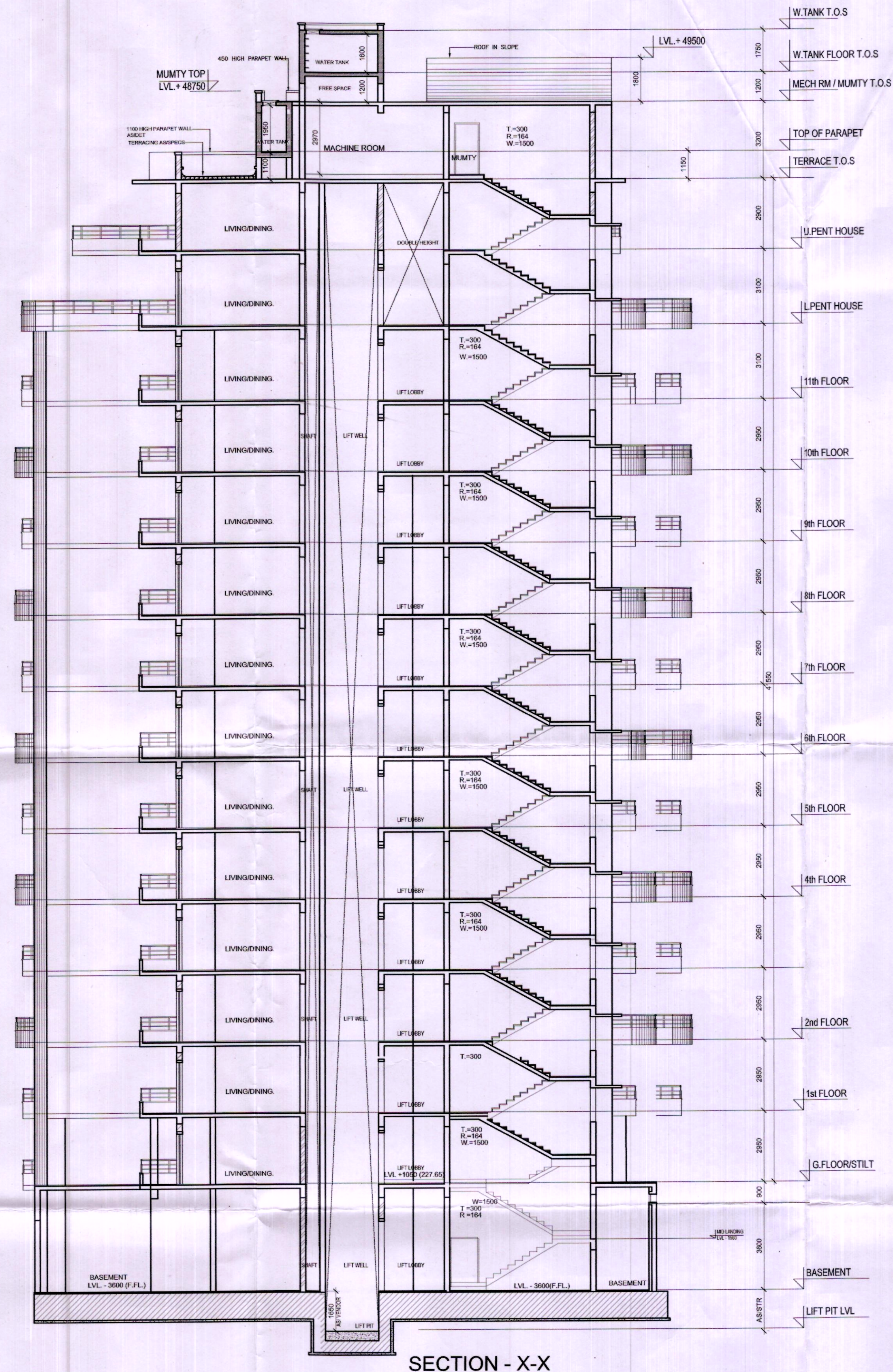
SECTION - X-X
