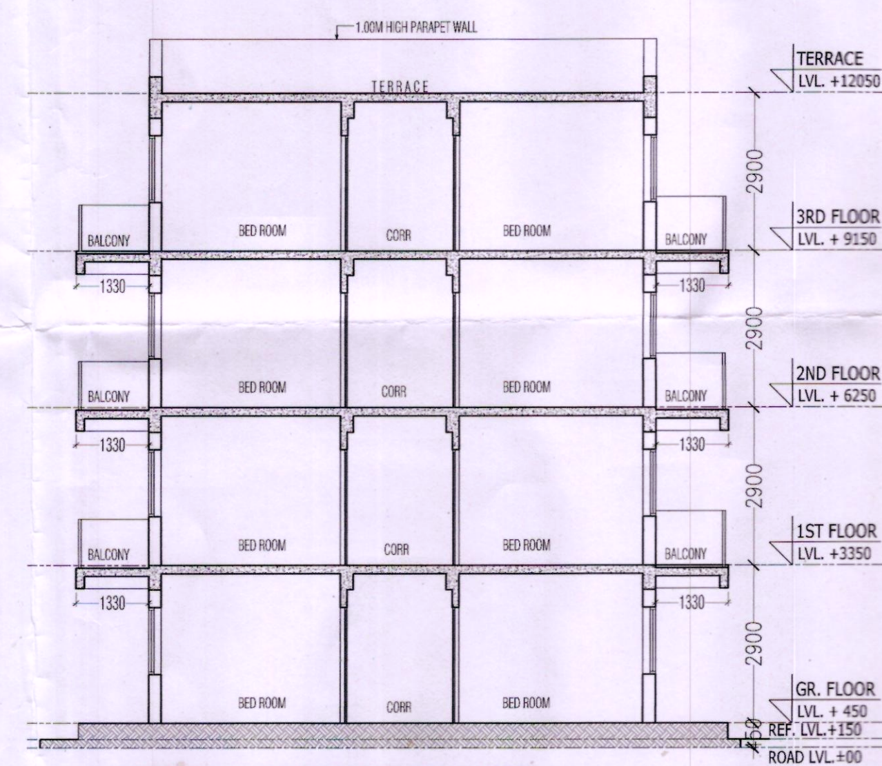
SECTION B-B EWS (BLOCK-A)
