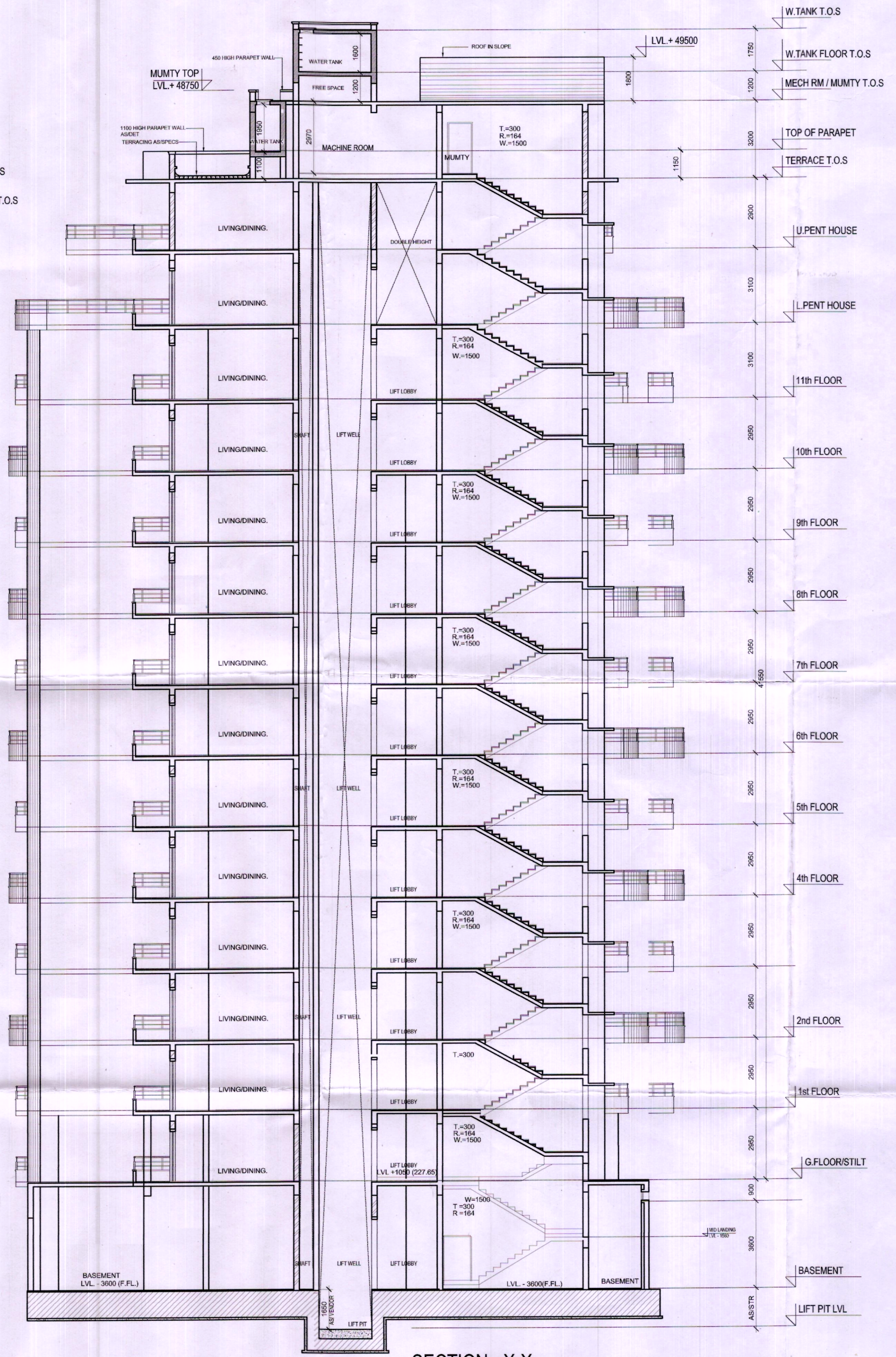
SECTION - X-X
