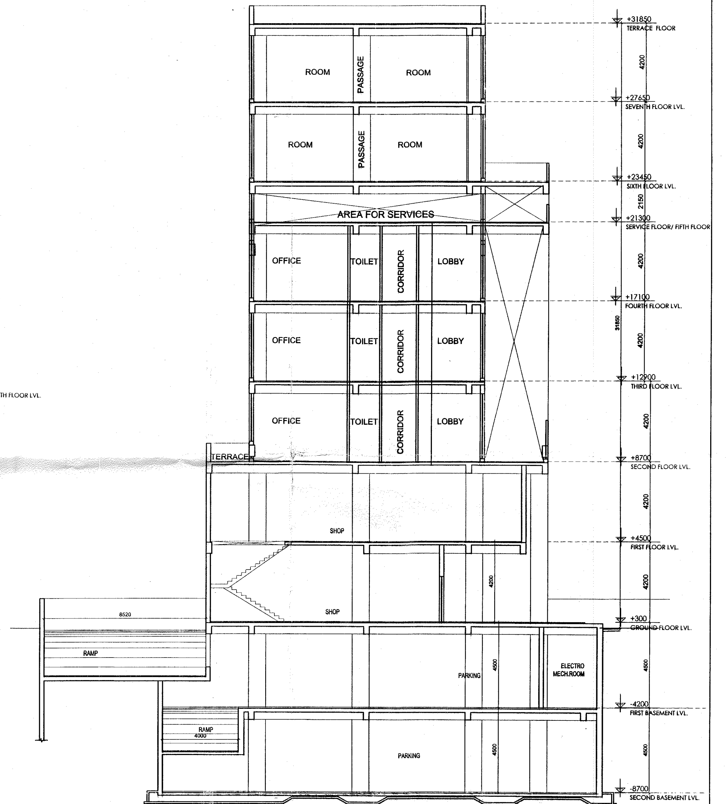
SECTION B-B
