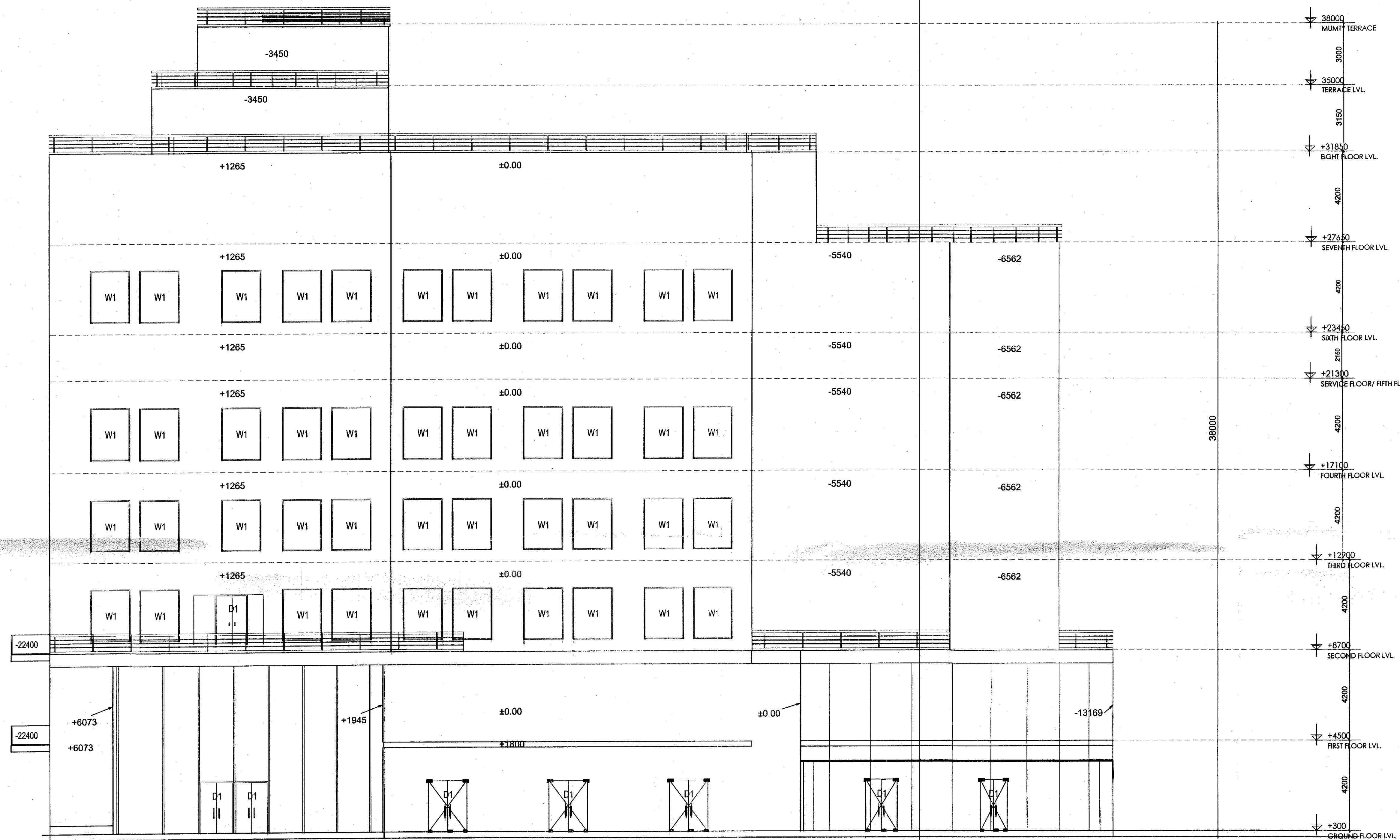
ELEVATION - 'A'
