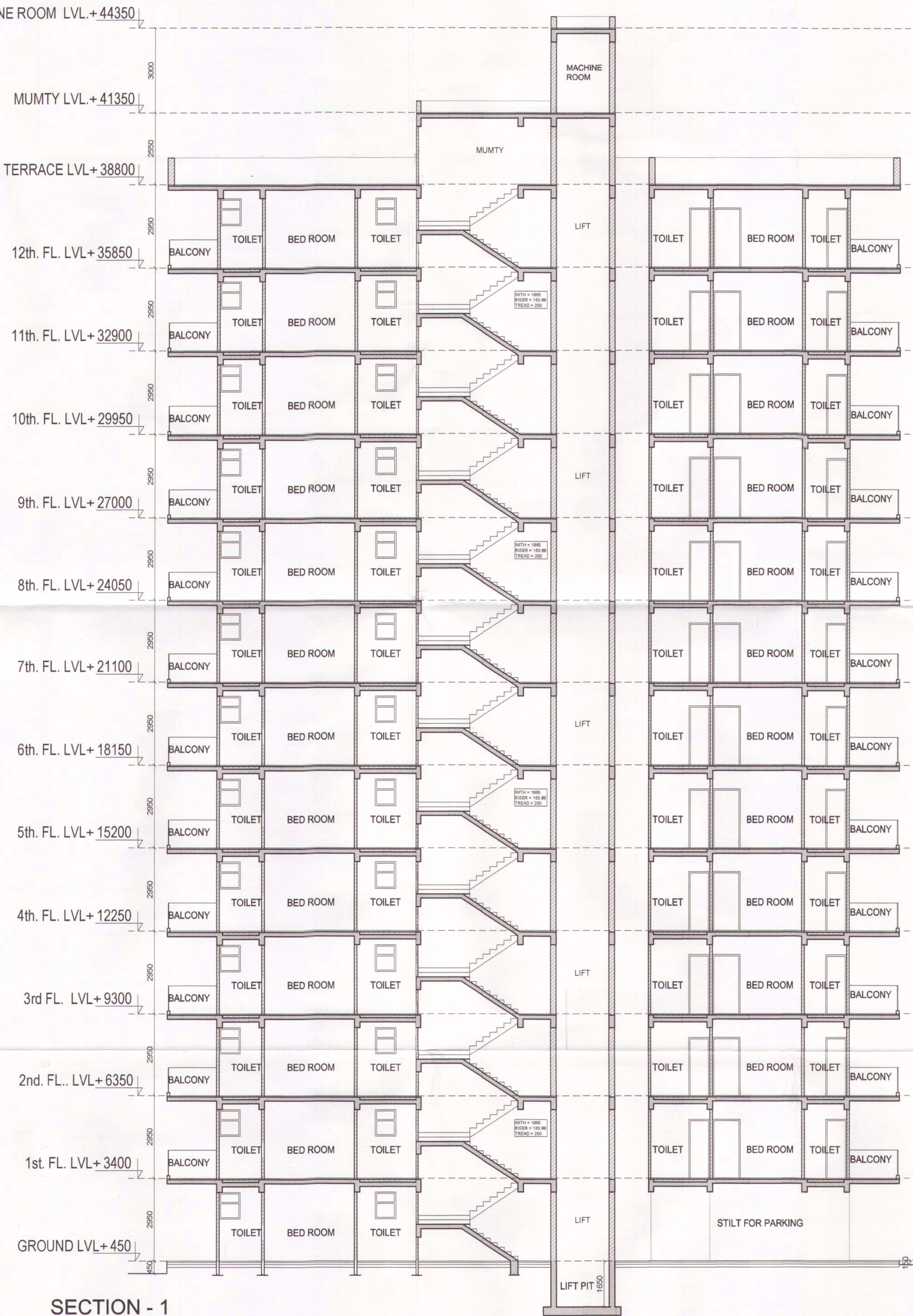
SECTION - 1
