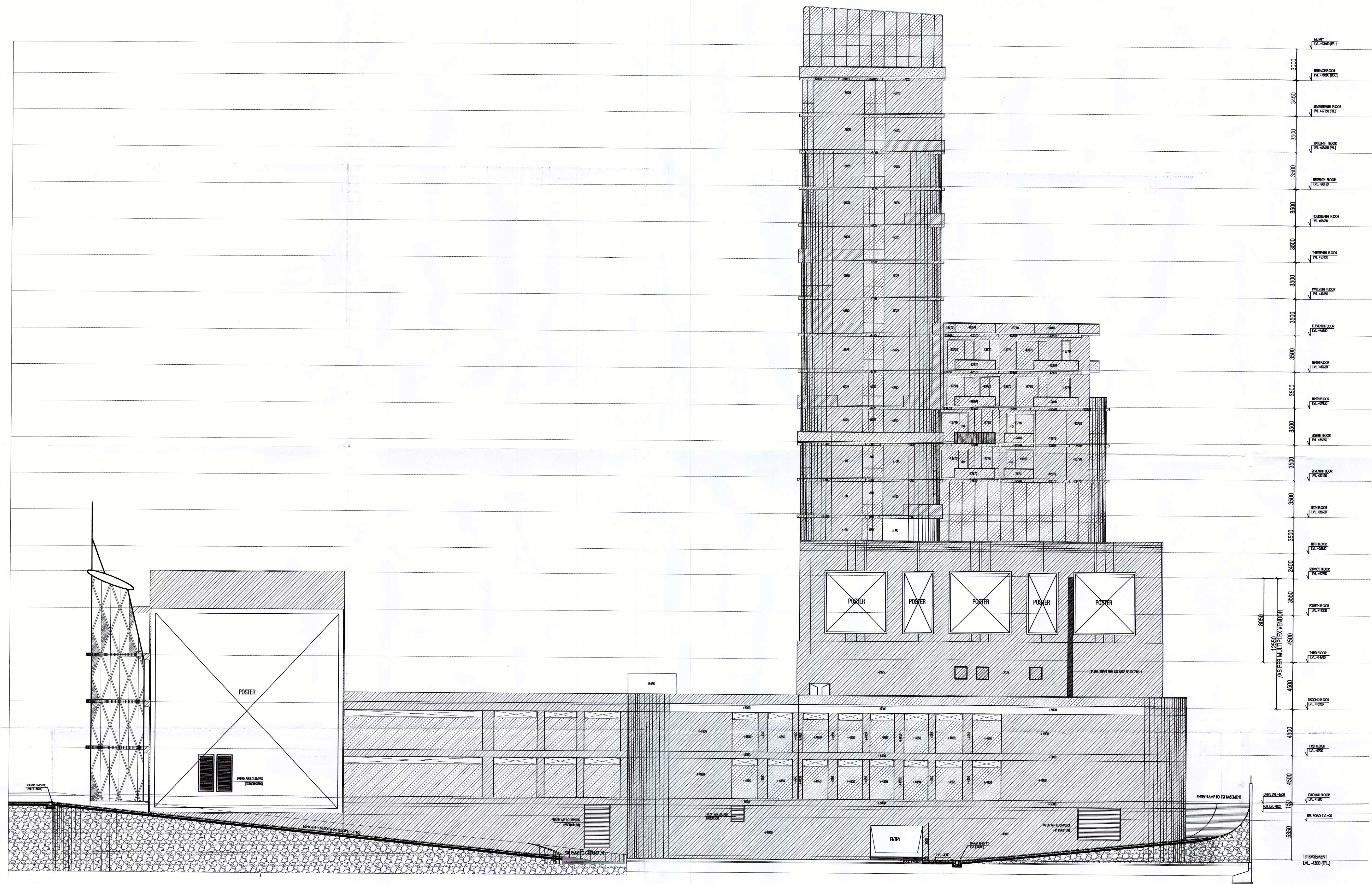
REAR ELEVATION
