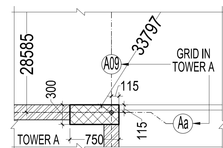
DETAIL B
