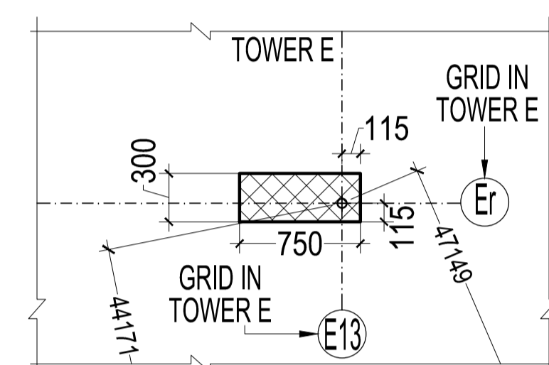
DETAIL C
