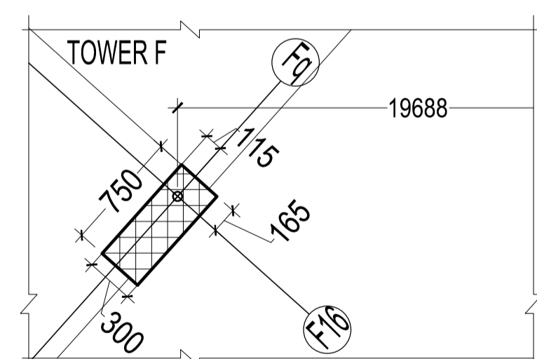
DETAIL H
