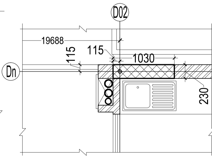
DETAIL I
