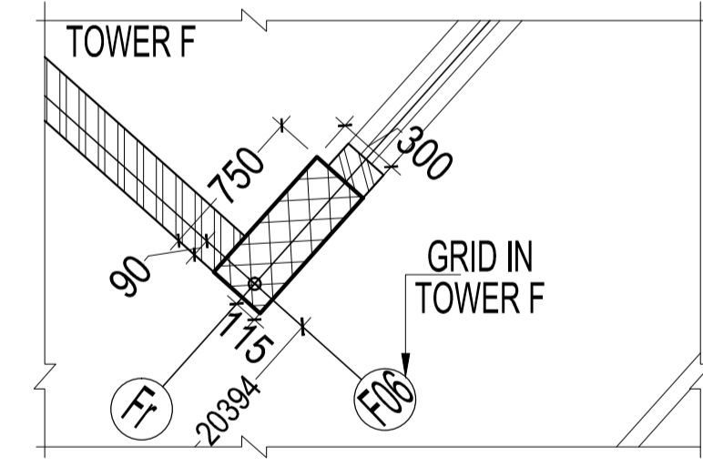
DETAIL E
