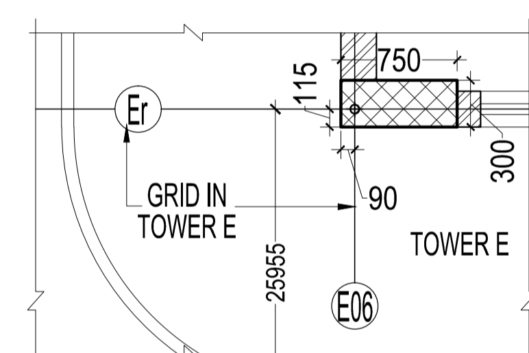
DETAIL D
