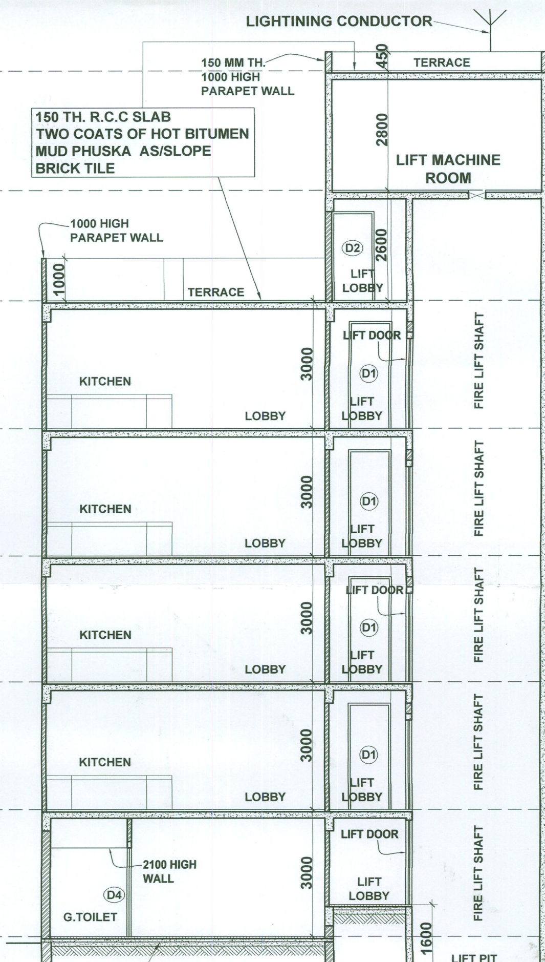
SECTION - 2-2
