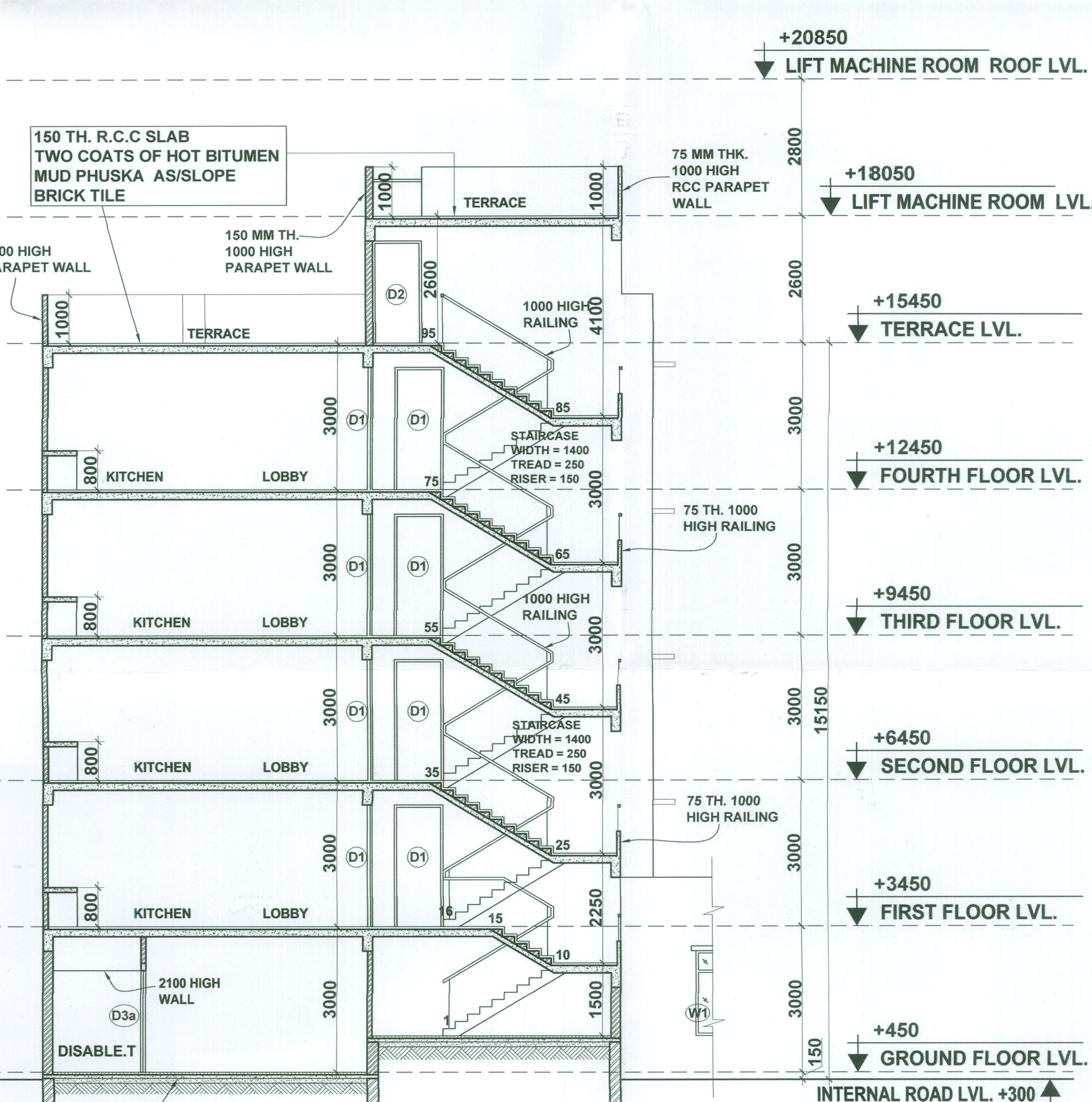
SECTION - 3-3
