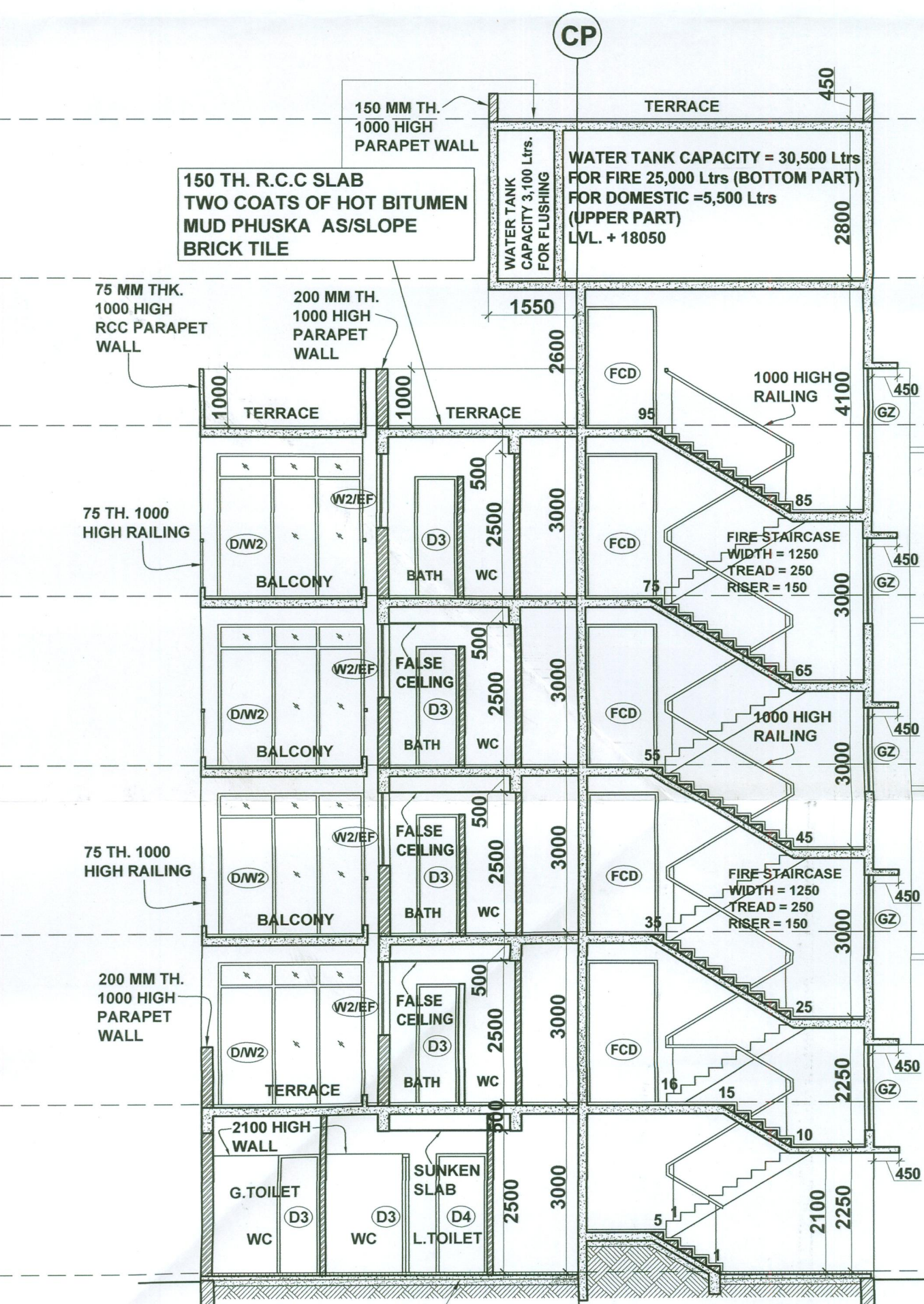
SECTION - 1-1
