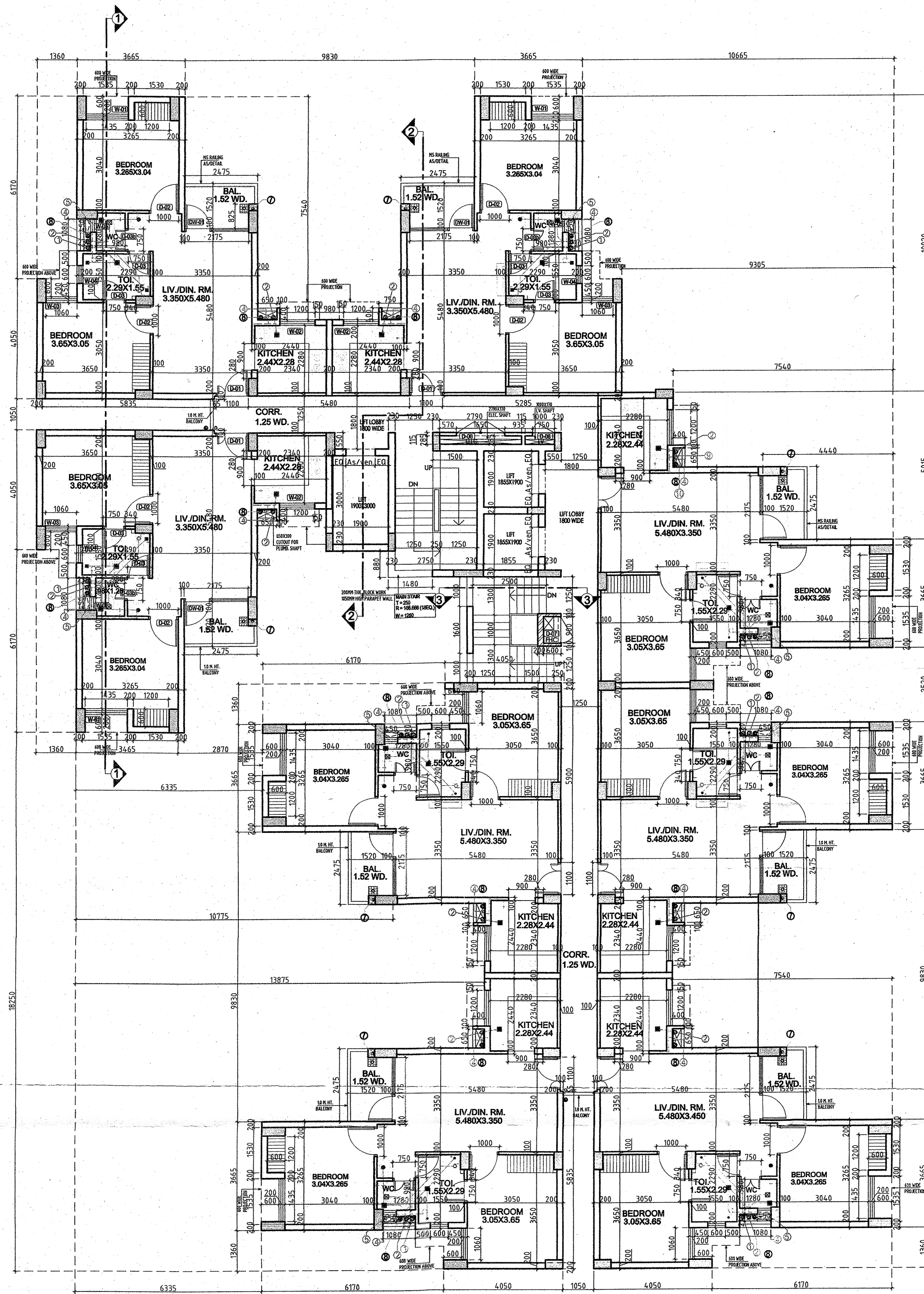
1st to 10th Floor Plan (Block-A & B)
