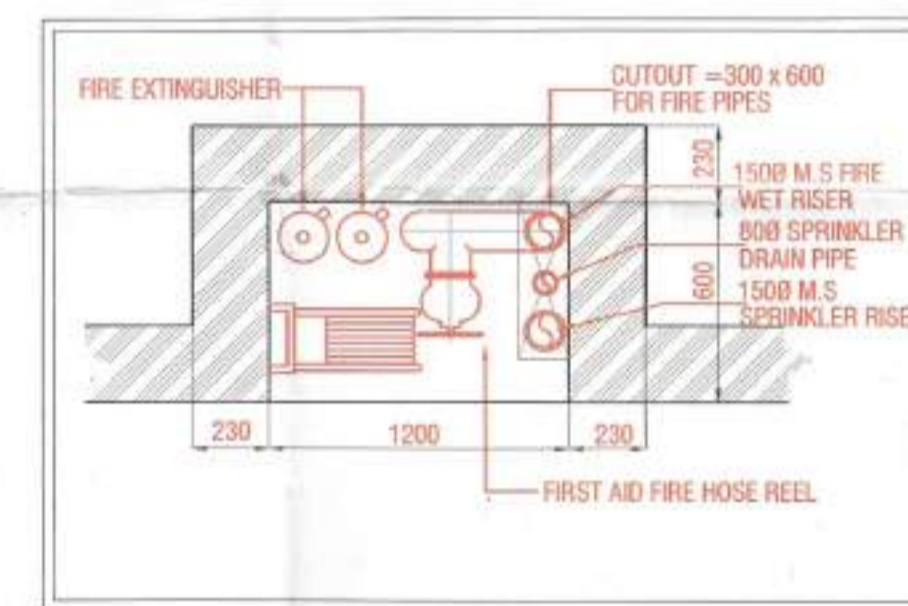
DETAIL OF FIRE HOSE CABINET (F.H.C.)
