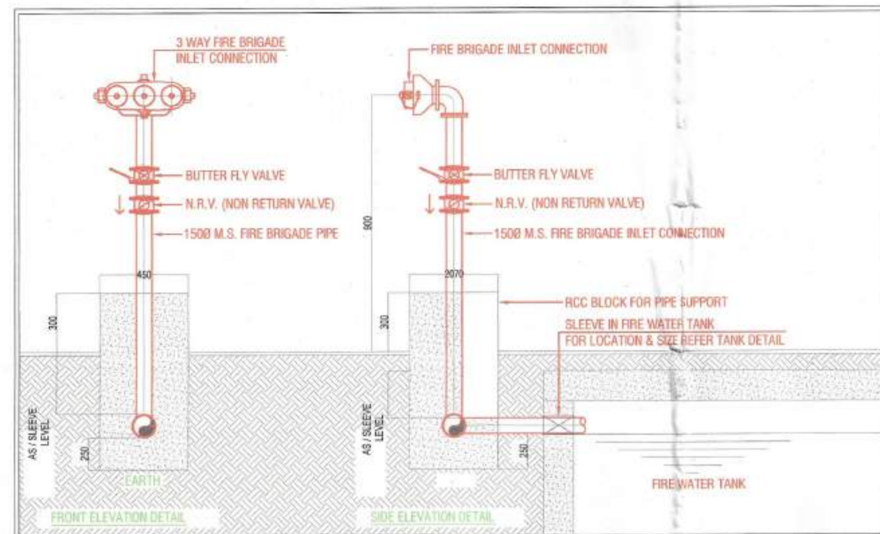
FIRE BRIGADE INLET CONNECTION DETAIL IN TANK (FRONT & SIDE)
