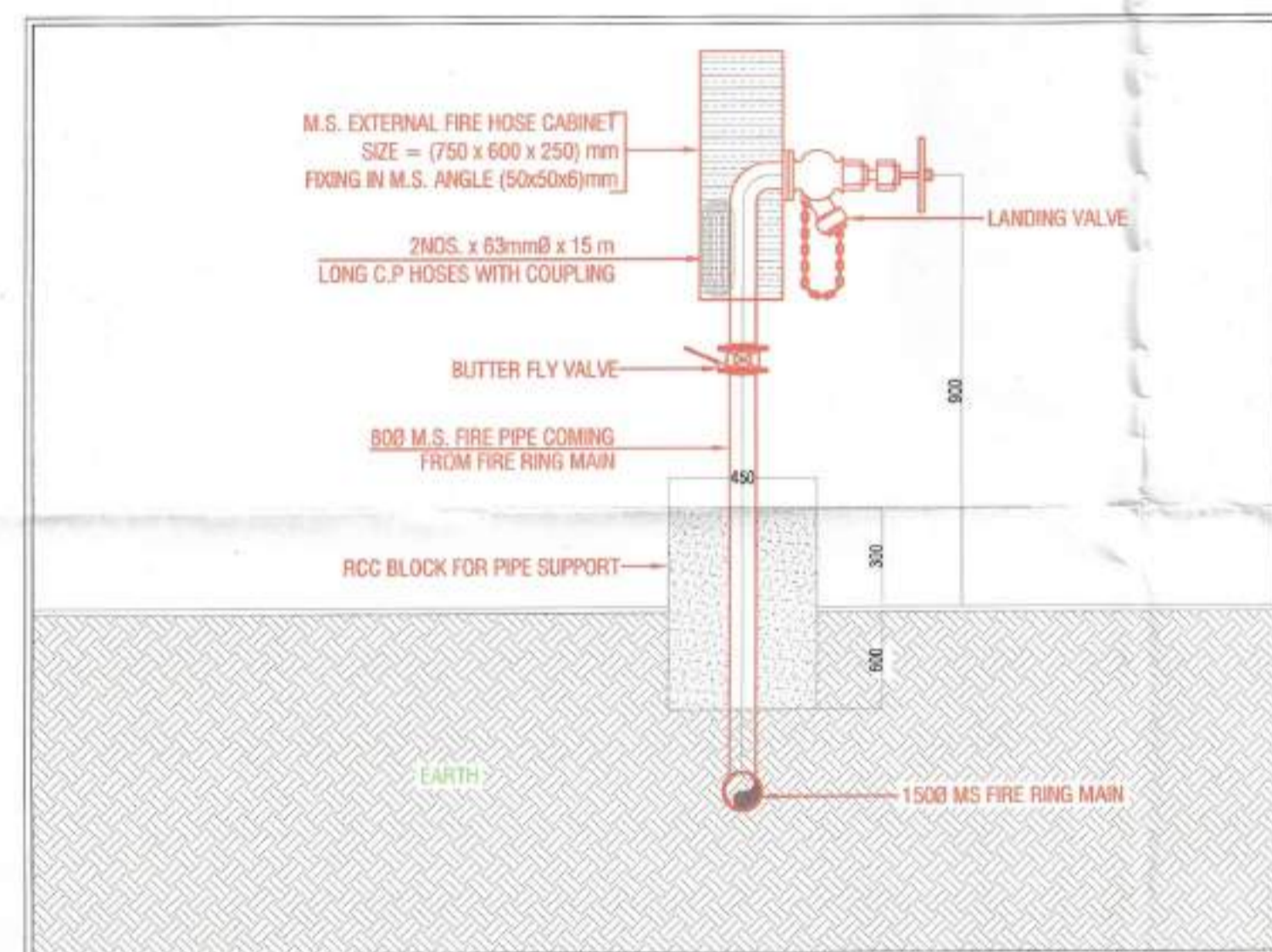
EXTERNAL FIRE HYDRANT SIDE ELEVATION DETAIL
