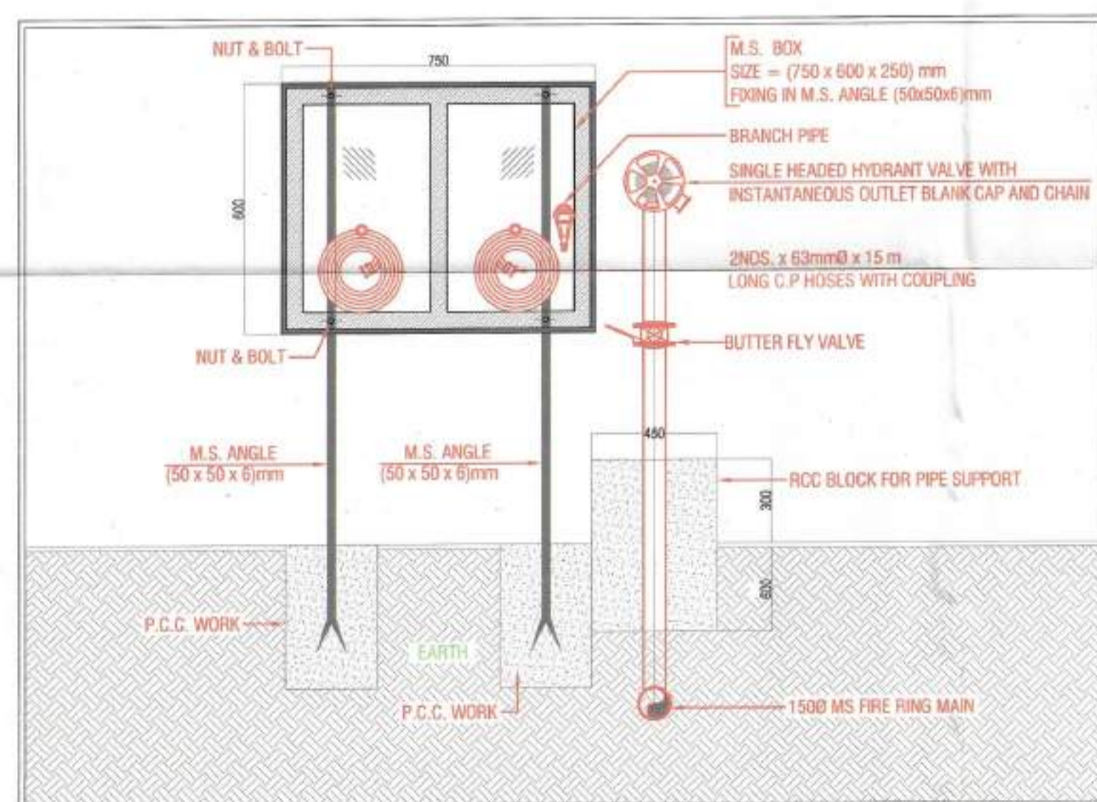
EXTERNAL FIRE HYDRANT FRONT ELEVATION DETAIL
