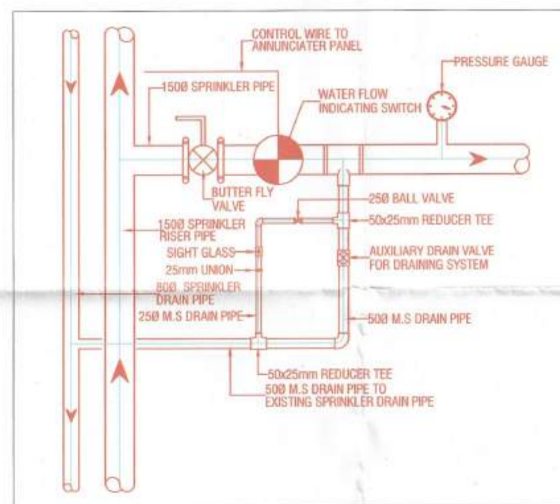
DETAIL OF FLOW INDICATING SWITCH
