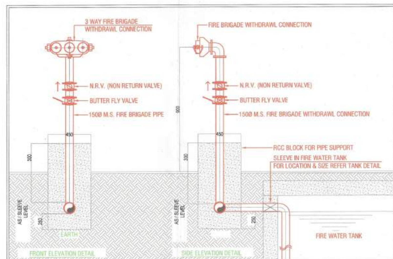
FIRE BRIGADE WITHDRAWAL CONNECTION DETAIL IN TANK (FRONT & SIDE)
