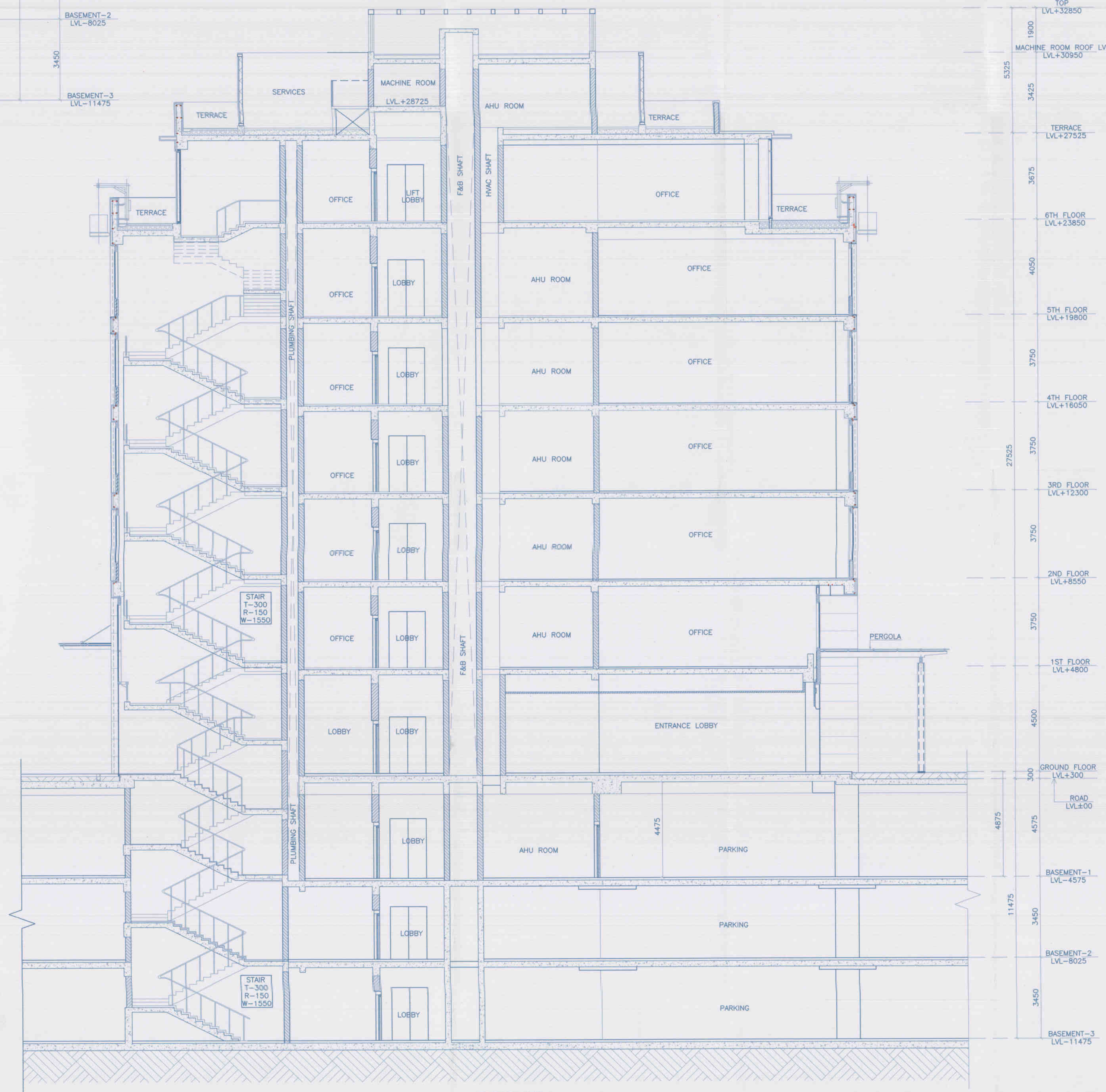
SECTION-BB (BLOCK-03)
