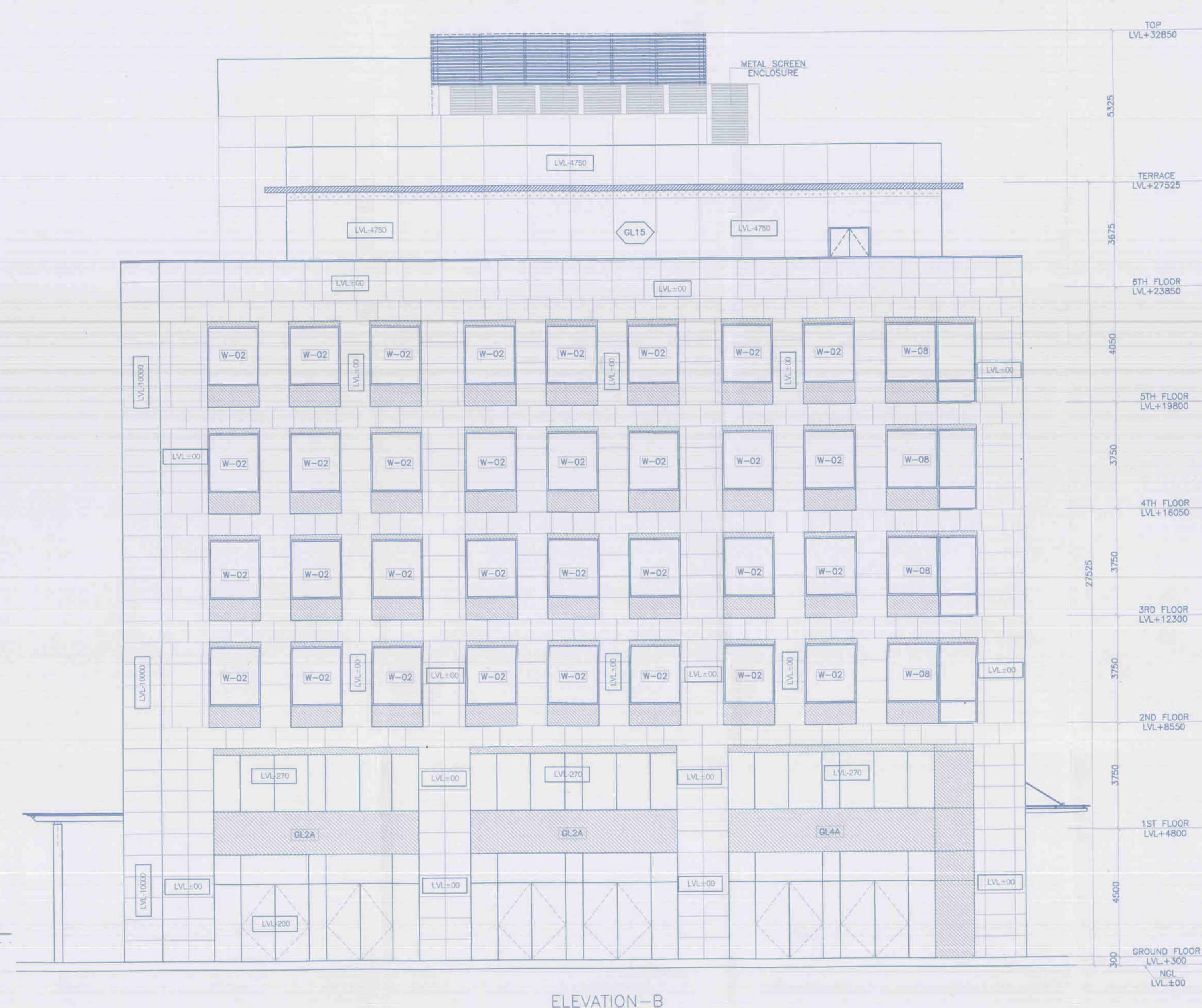
ELEVATION-B (BLOCK-5)
