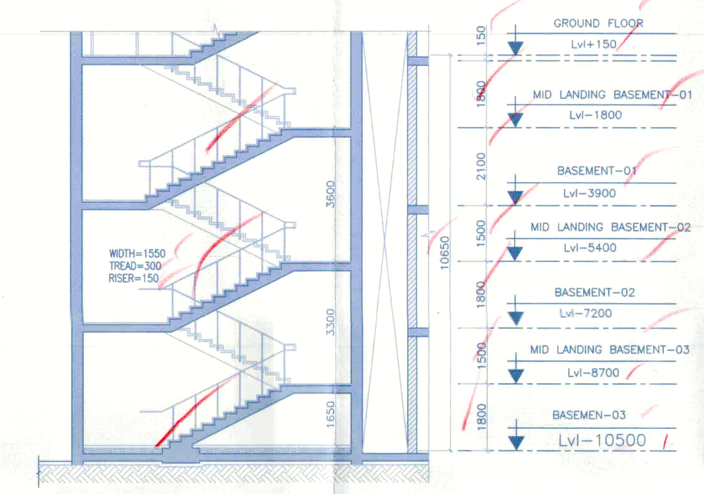
OFFICE TOWER STAIRCASE SECTION-05
