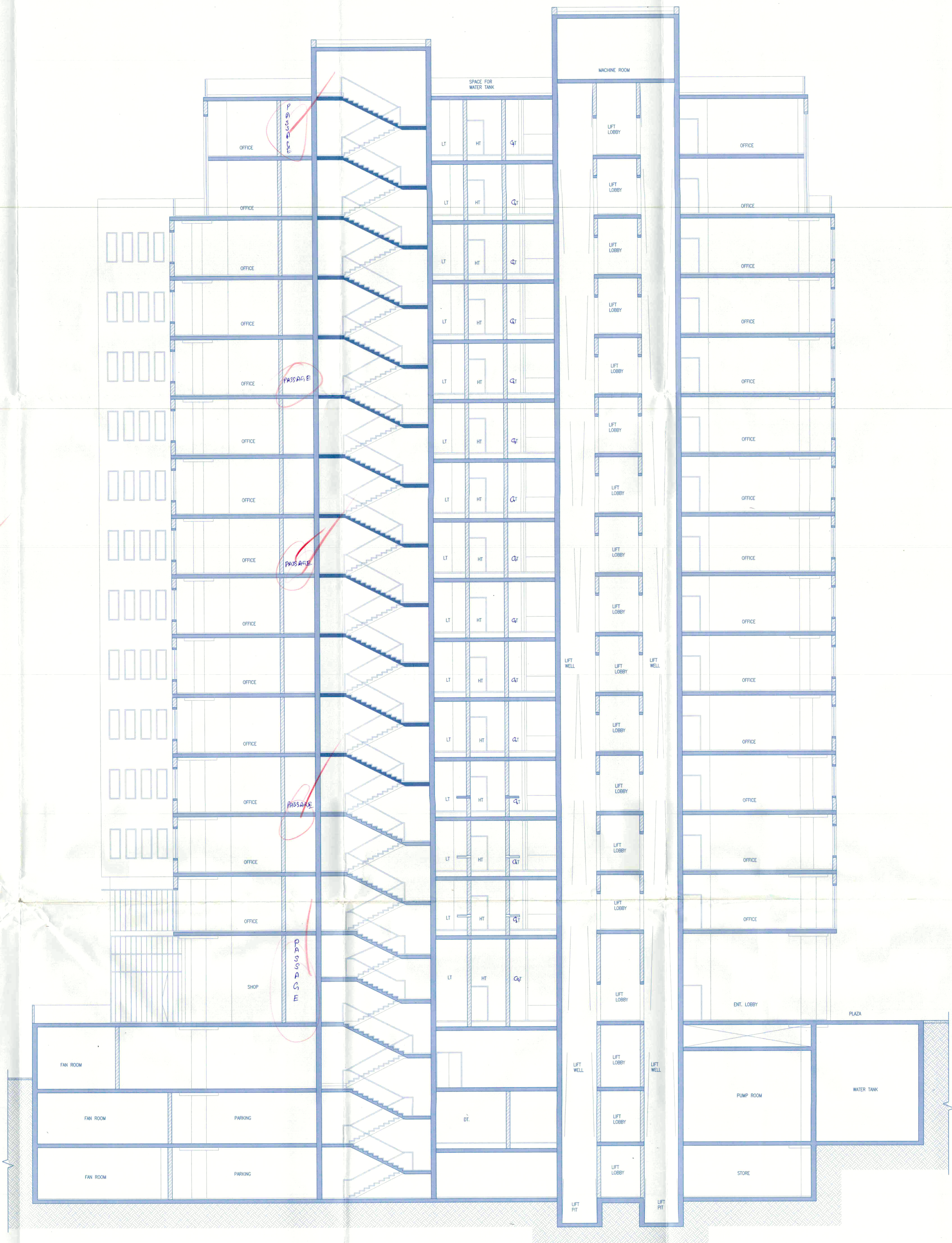
OFFICE TOWER SECTION-02
