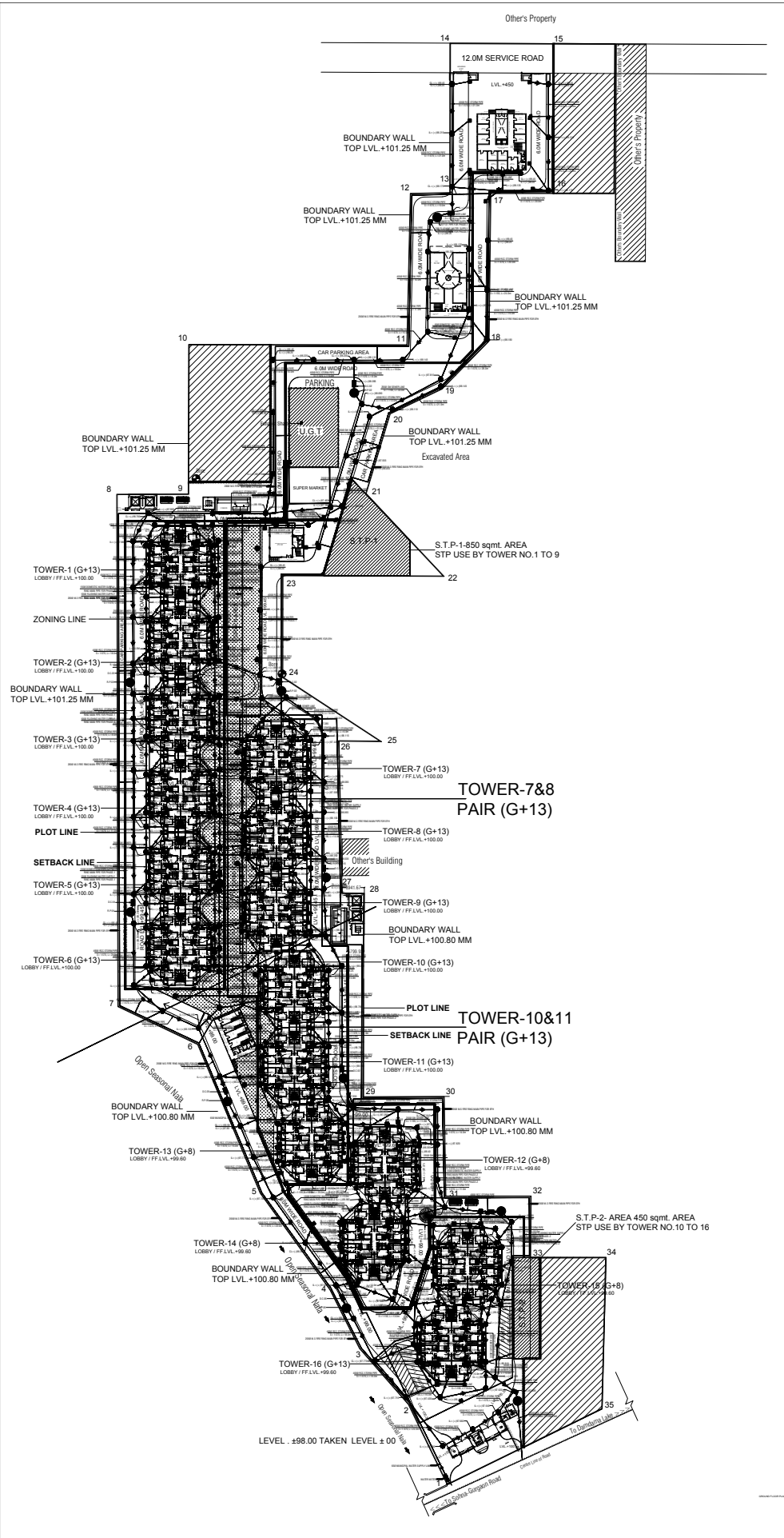
GROUND FLOOR PLAN SITE PLAN LEVEL . ±99.00 TAKEN LEVEL ± 00
