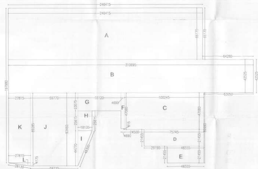
BASEMENT FLOOR AREA DETAIL PLAN SCALE 1:1000
