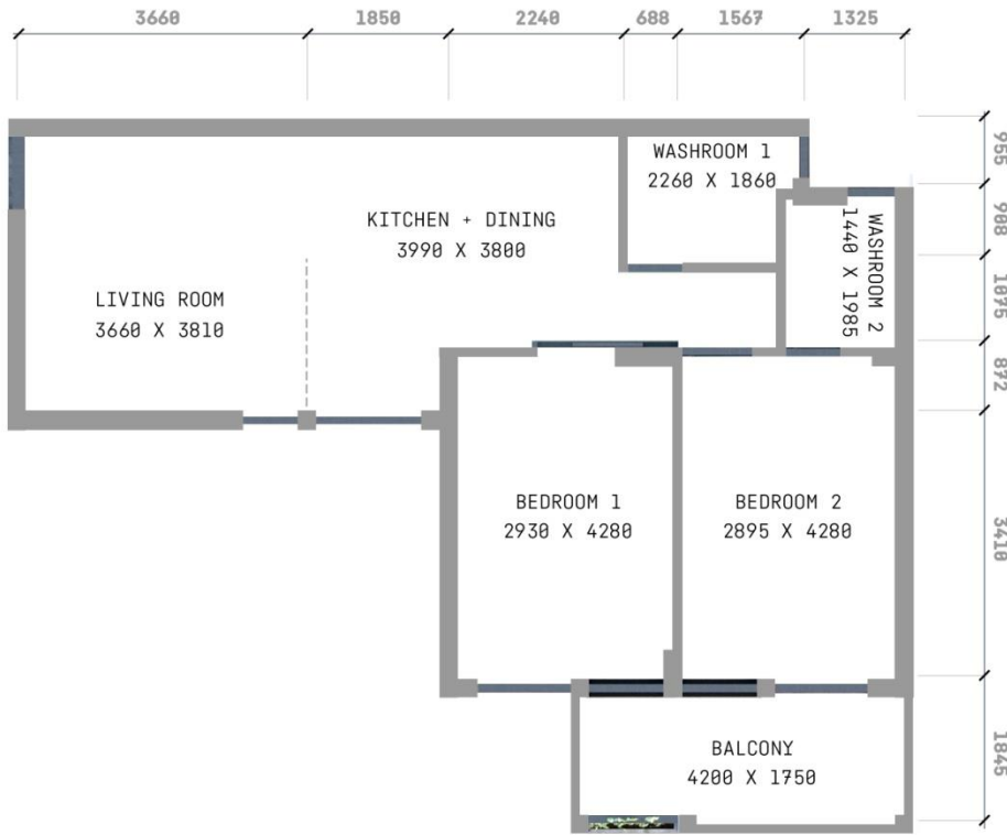
Floor Plan of the Project "OUR HOMES 3"
