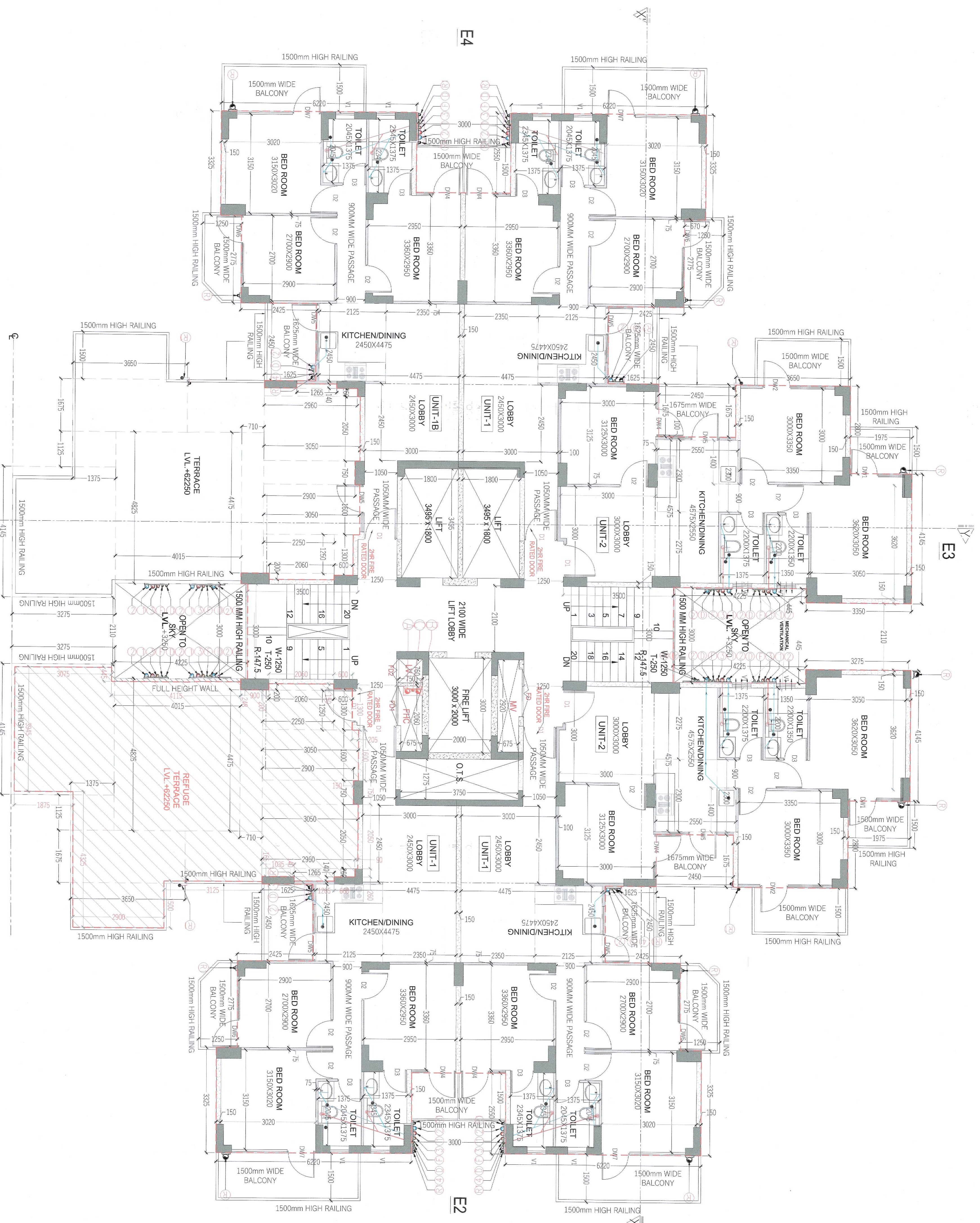
21ST FLOOR PLAN TOWER- F LVL-662250
