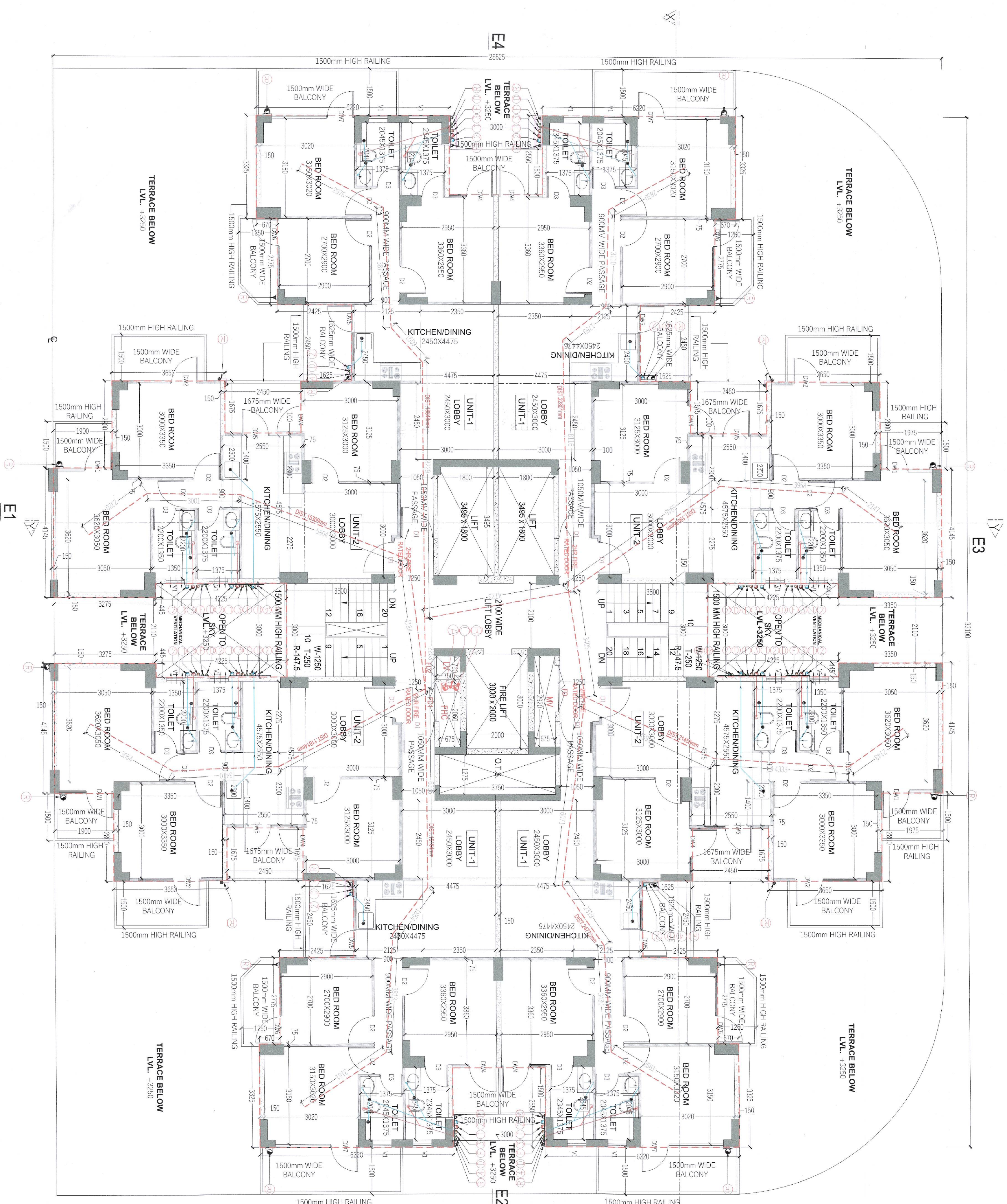
TYPICAL FLOOR PLAN 2ND TO 20TH TOWER-F
