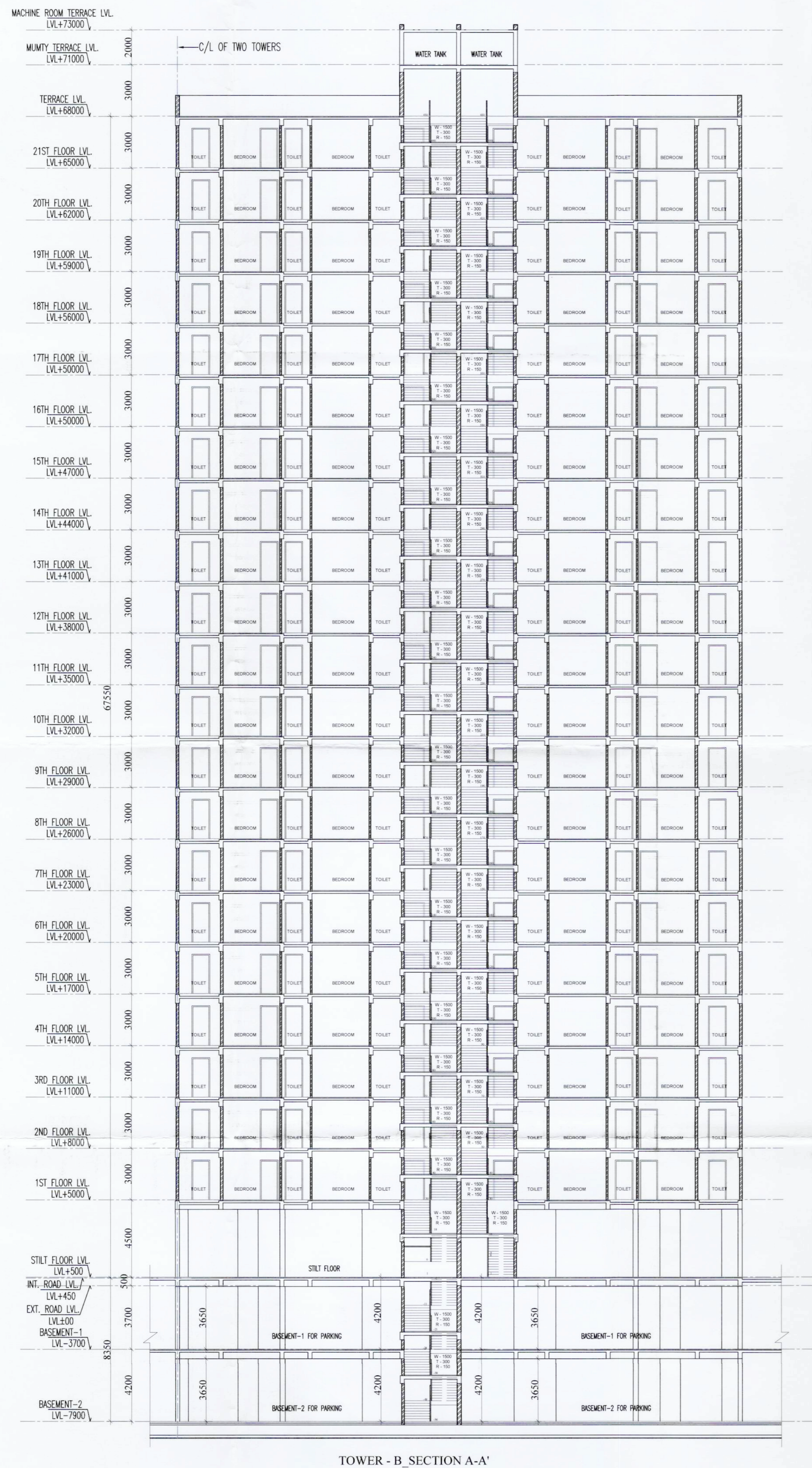
TOWER - B_SECTION A-A'
