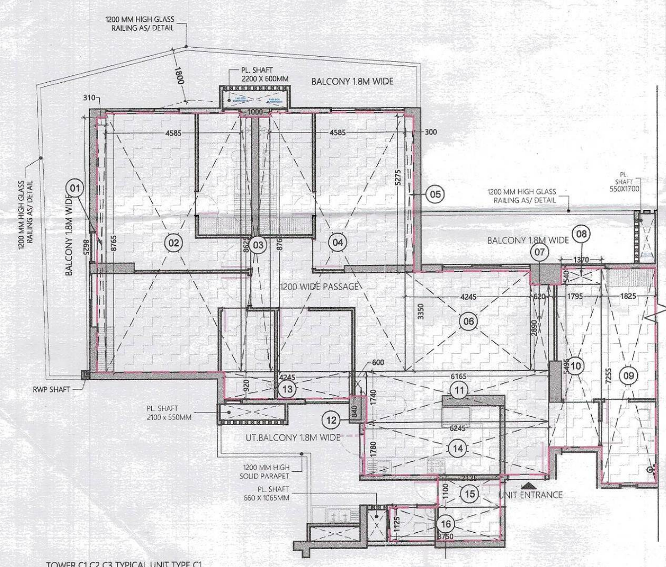
03A TOWER C1, C2 & C3 - TYPICAL UNIT (TYPE C1) REF: SCALE: 1:100
