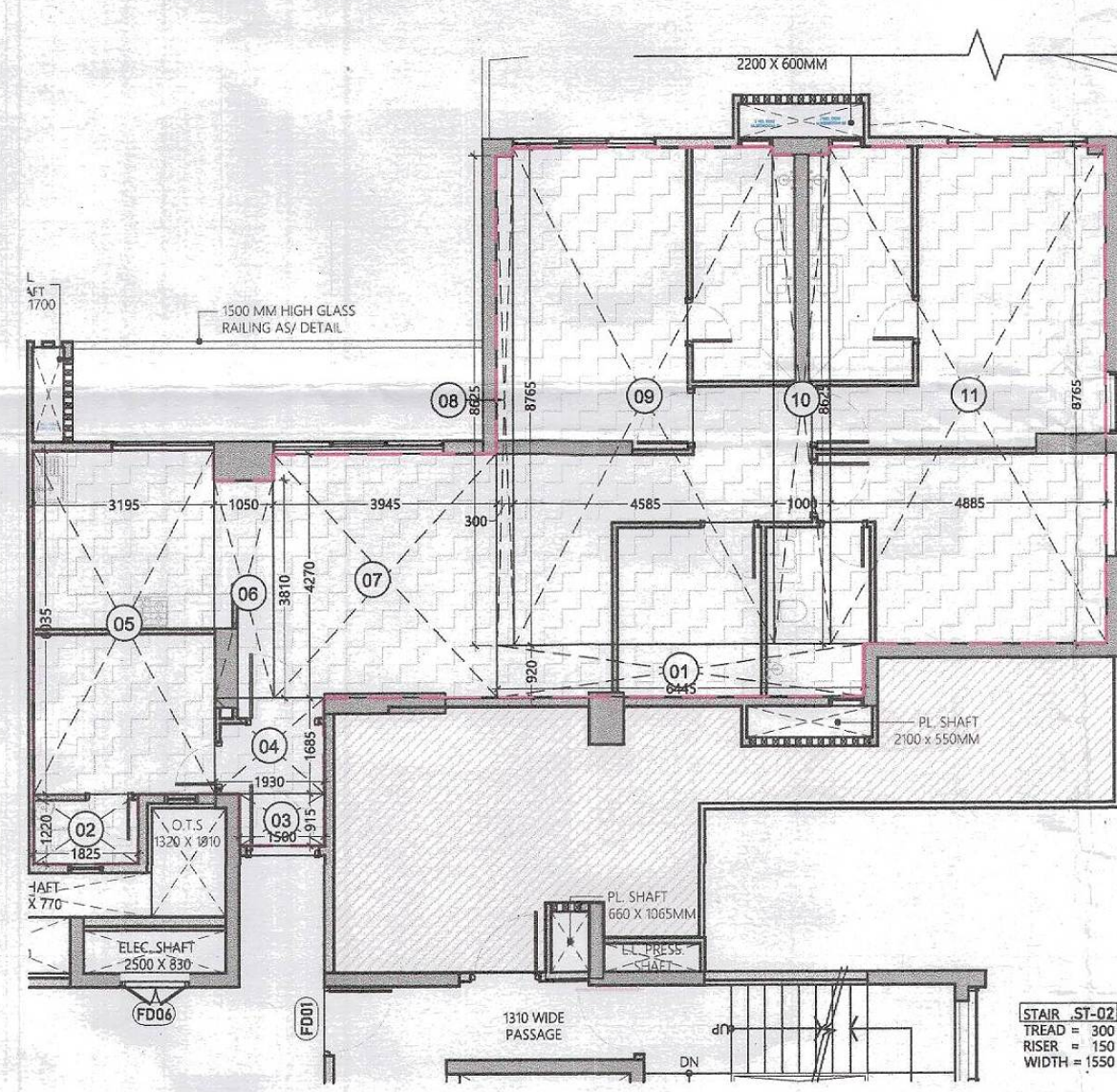
03B TOWER C1, C2 & C3 - TYPICAL UNIT (TYPE C2) REF: SCALE: 1:100
