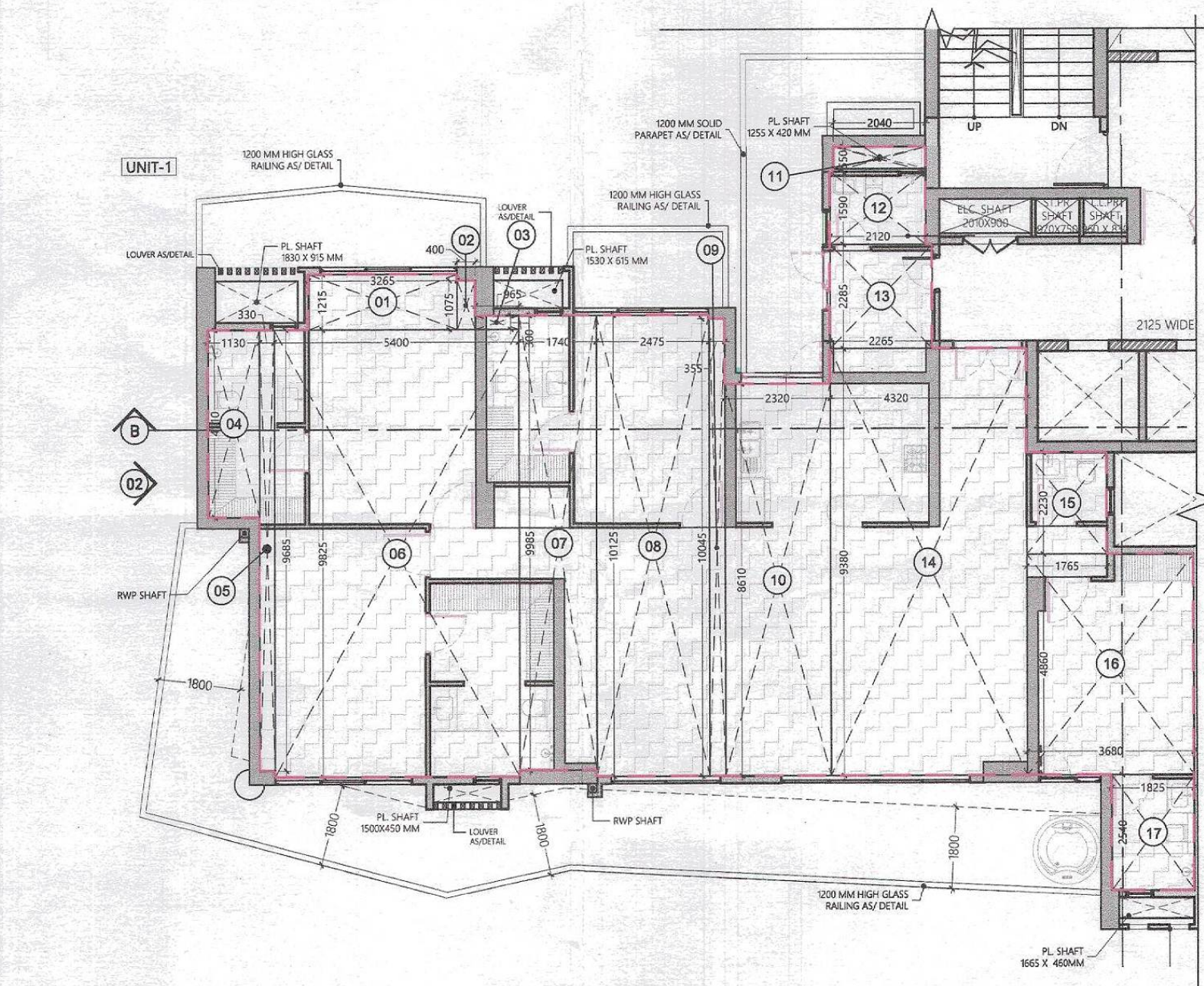
02A TOWER B1 & B2 - TYPICAL UNIT PLAN (TYPE B) REF: SCALE: 1:100
