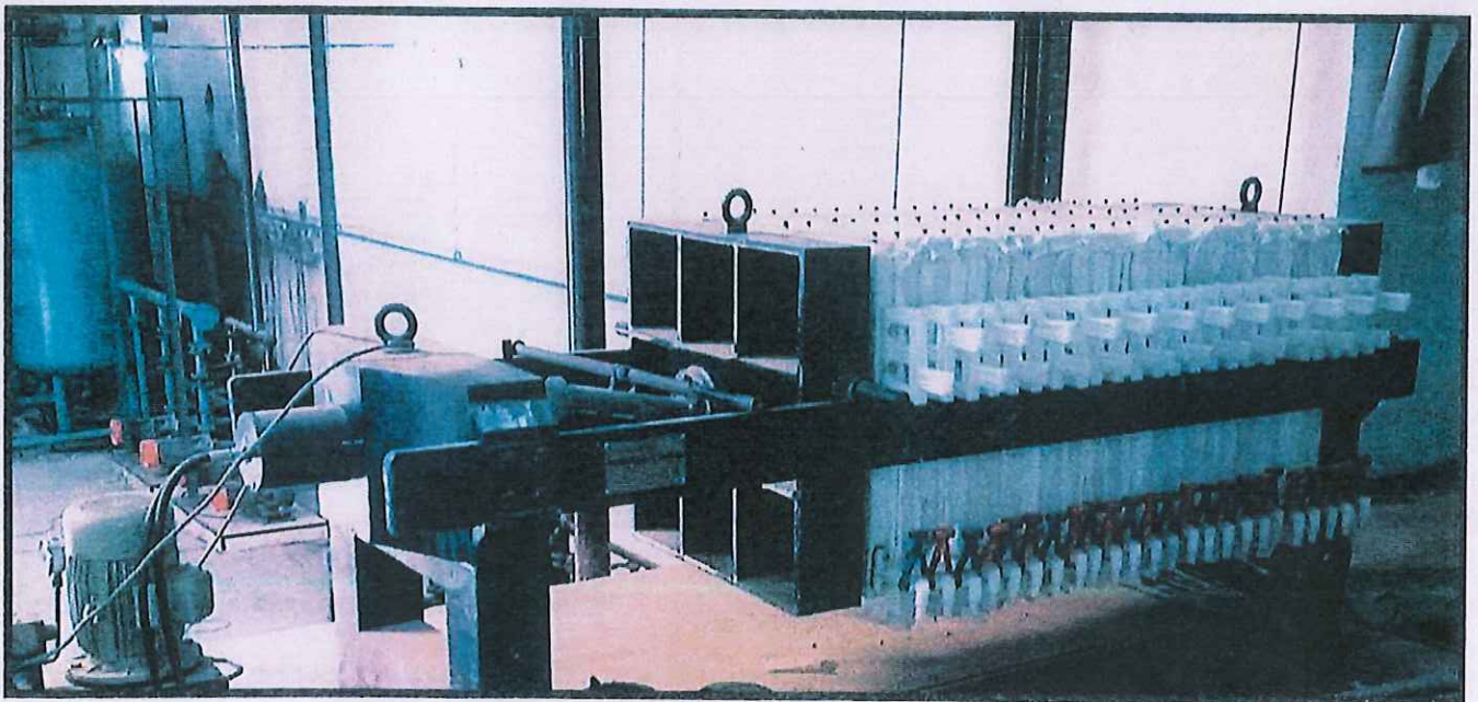
Filter Press
