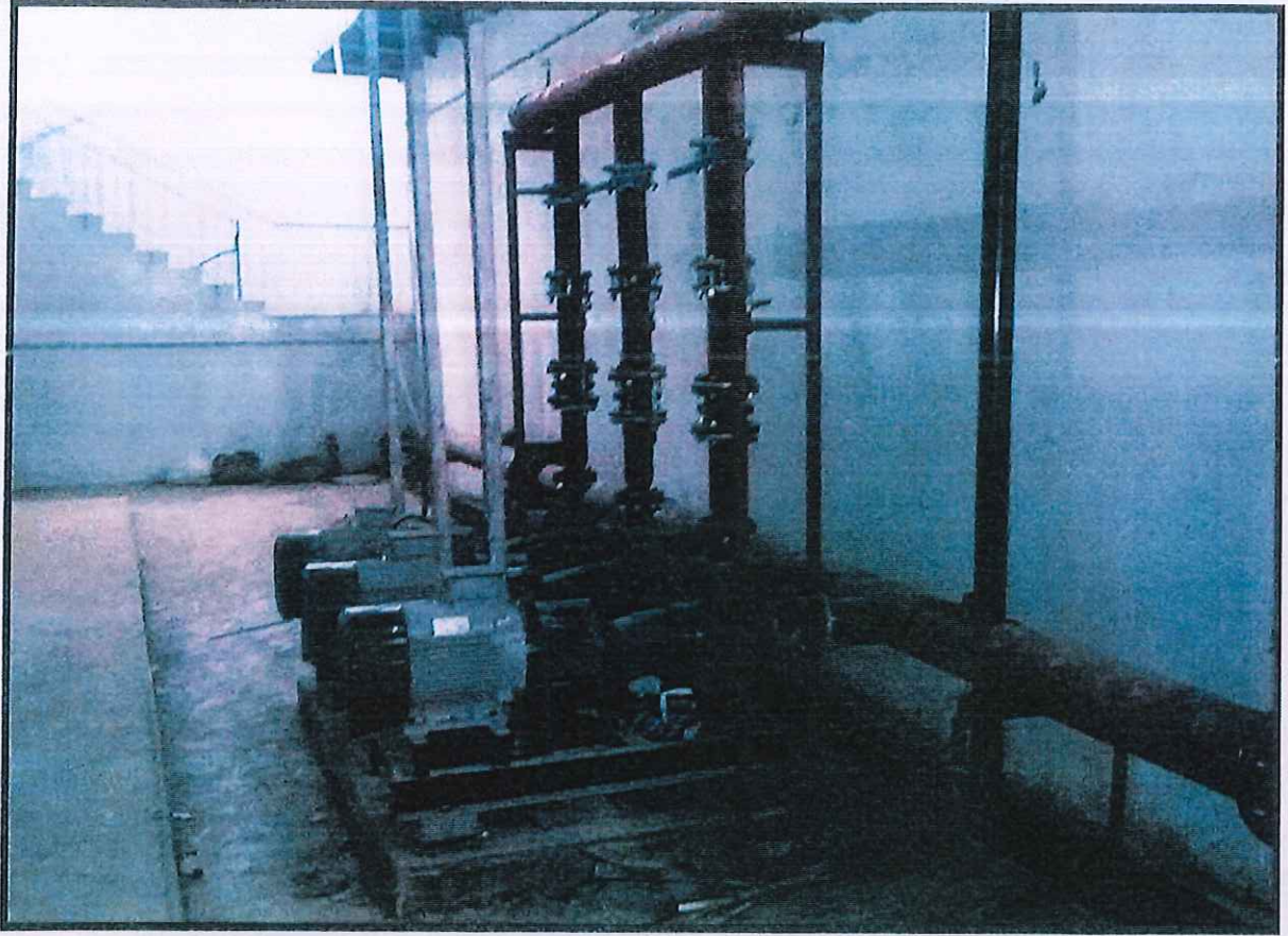
Recycled Water Pumps
