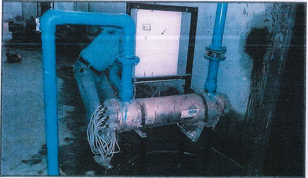
Ultra Violet Disinfection System
