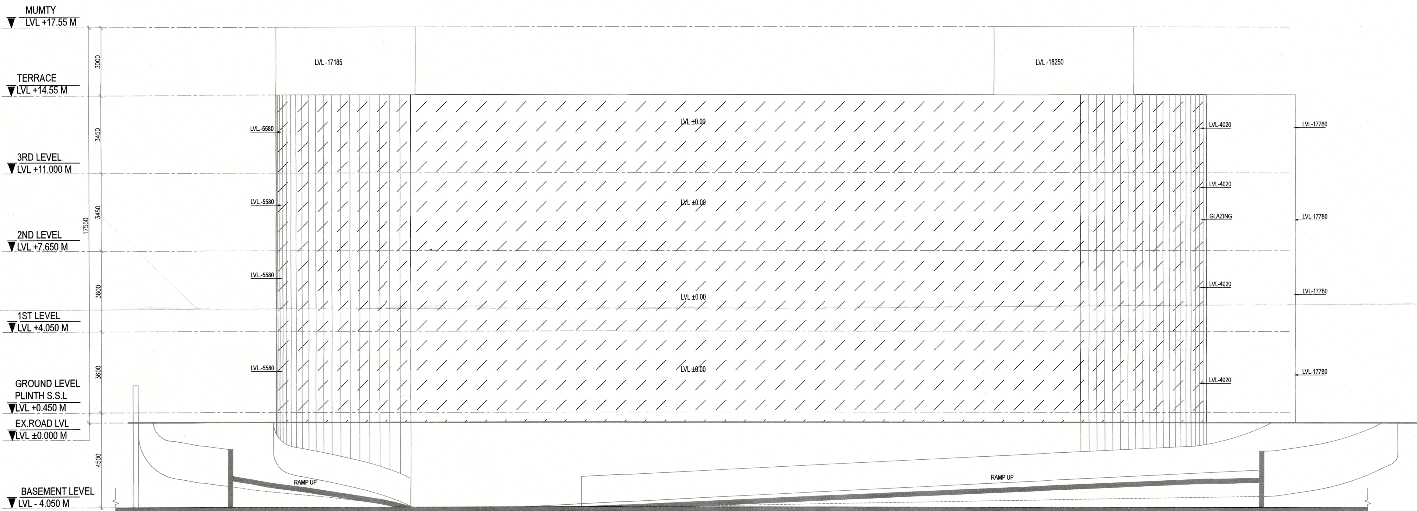
ELEVATION Y-SIDE
