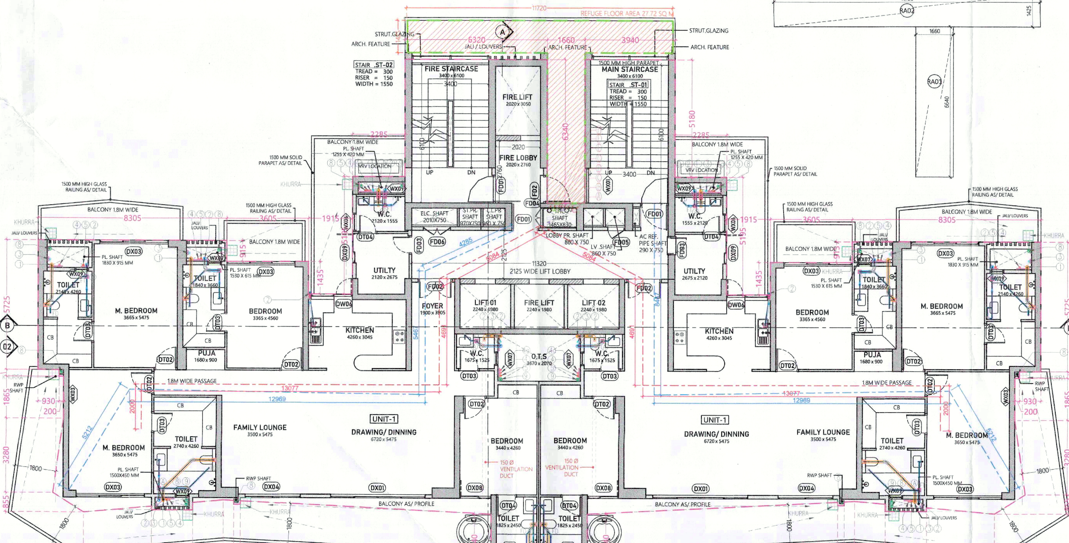
TOWER-B2 16TH FLOOR PLAN : LVL +62400
