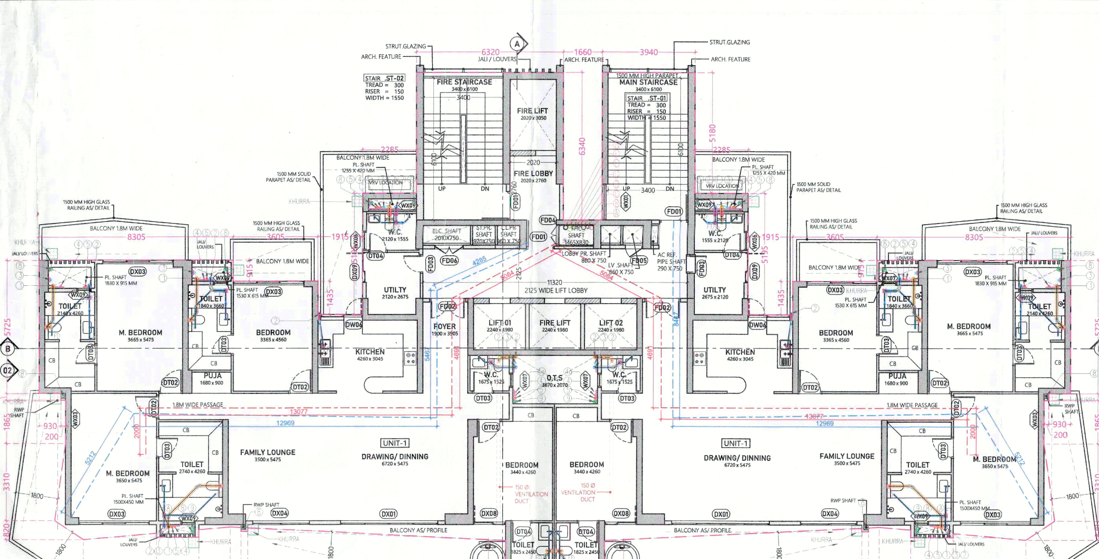
TOWER-B2 14TH FLOOR PLAN : LVL +55200 & 15TH FLOOR PLAN : LVL +58800
