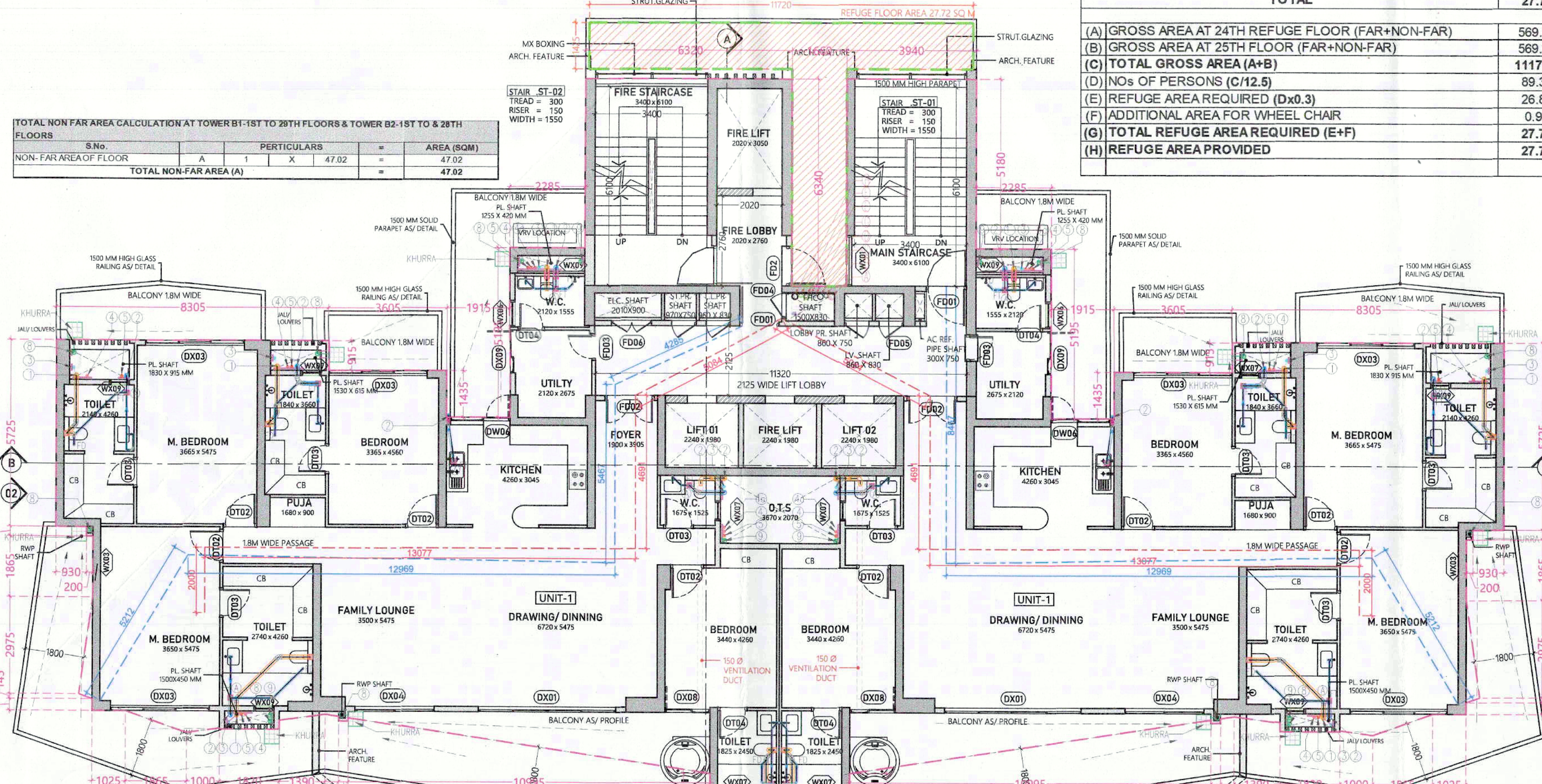
TOWER-B2 24TH FLOOR PLAN : LVL +91200
