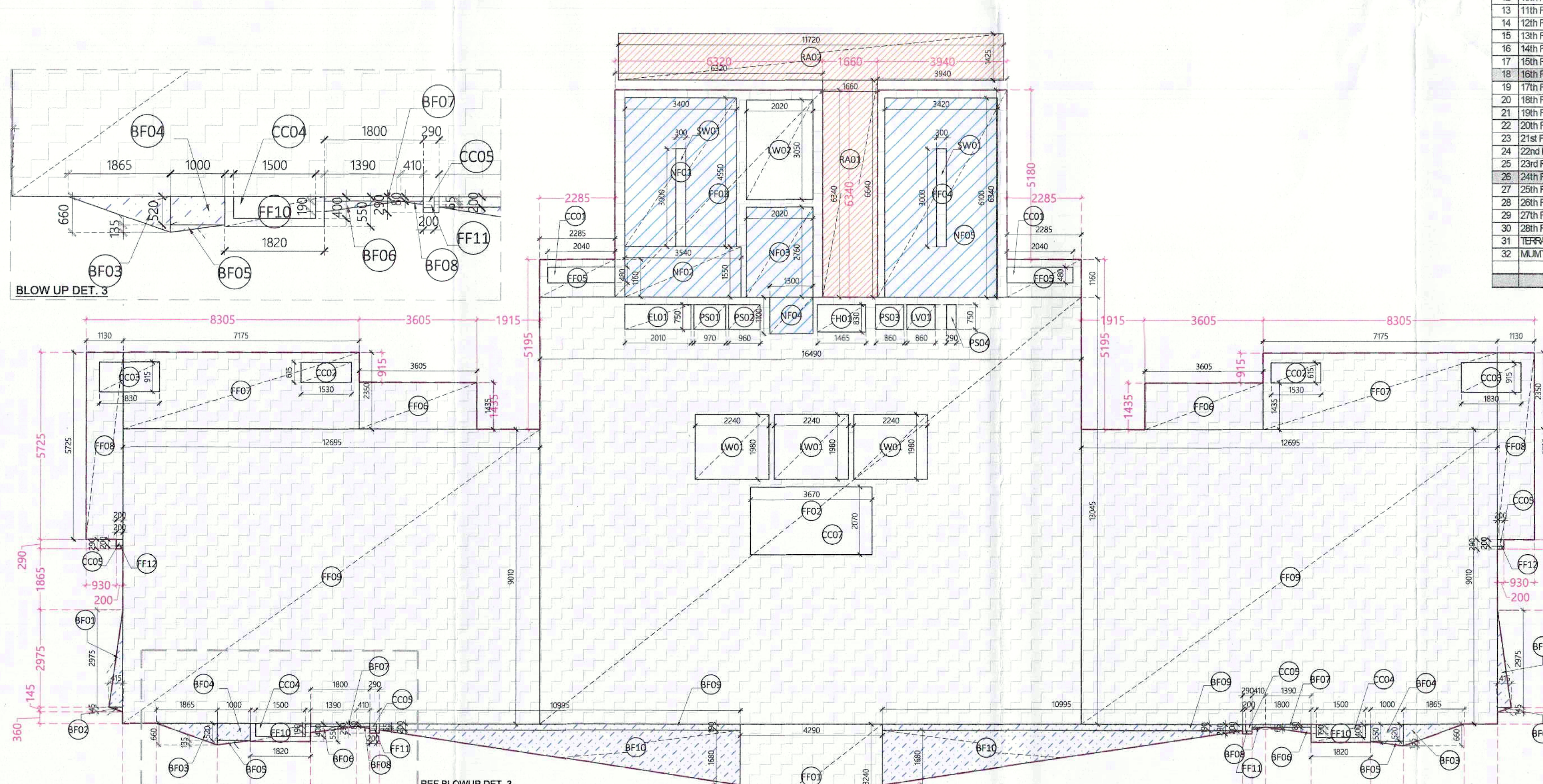
TOWER-B2 24TH FLOOR AREA DIAGRAM
