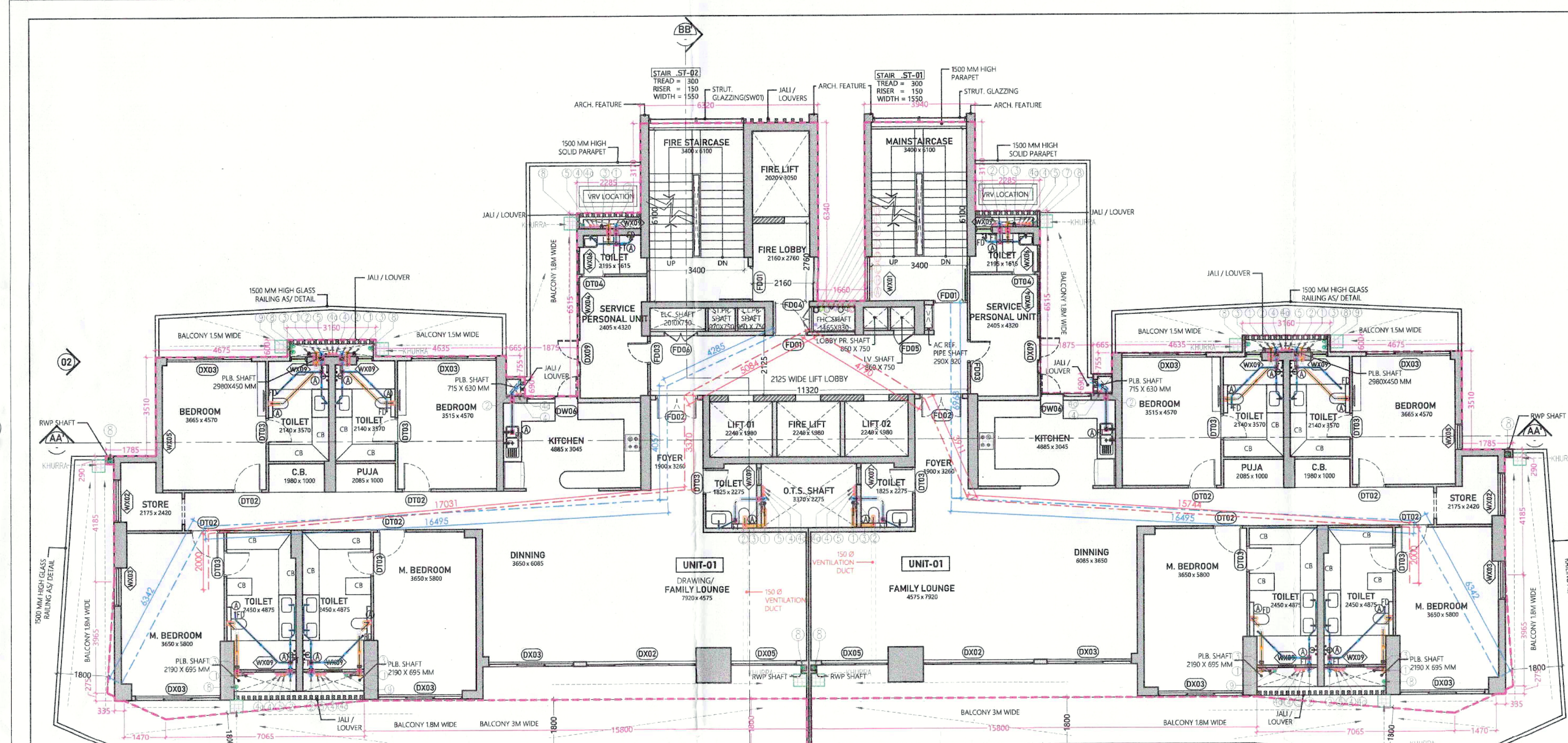
8TH FLOOR PLAN : LVL +33600MM 22TH FLOOR PLAN : LVL +84000 MM
