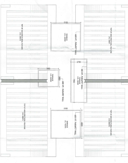
ROOF PLAN (TOWER-B)
